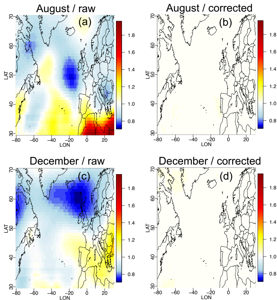
Figure A2. (a) Mean ratio of standard deviation of Z500 bias of 11 CMIP6 simulations for August. (b) Mean ratio of standard deviation of Z500 bias of 11 CMIP6 simulations after bias correction for August. (c) Mean ratio of standard deviation of Z500 bias of 11 CMIP6 simulations for December. (d) Mean ratio of standard deviation of Z500 bias of 11 CMIP6 simulations after bias correction for December.
