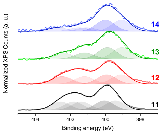
Fig. 2 High resolution N_{1s} spectra of TPIL dynamic networks 11–14 . The spectra are shifted vertically for clarity. The extents of N -alkylation reaction ( x ) are calculated from the 1,2,3-triazolium:1,2,3-triazole area ratios as discussed in the text (eq. 1). Please note that overlapping of Gaussian signals are indicated by darker shades.
