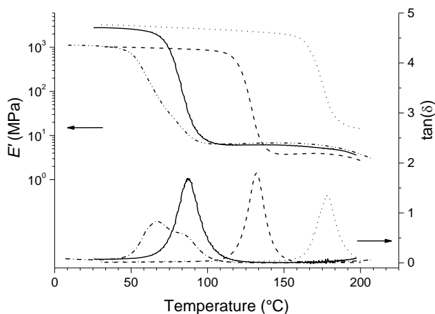
Fig. 3 DMA traces (1 Hz, 3 °C min -1 ) of TPIL dynamic networks 11 (solid lines), 12 (dashed lines), 13 (dotted lines) and 14 (dash-dotted lines).
