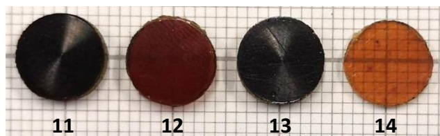
Fig. 1 Optical images of ca. 2 mm thick TPIL dynamic networks 11–14 (Dimensions of the tiles are 0.5 \times 0.5 \text{ cm}^2 ).
