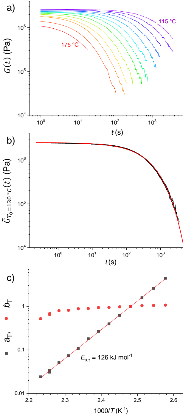
Fig. 4 a) Variable-temperature stress relaxation moduli of TPIL dynamic network 11 (from purple to red: 115 to 175 °C by +5 °C increments), and corresponding b) master curve and c) shift factors constructed at a reference temperature of T_0 = 130 °C. The red line in b) corresponds to a stretched exponential model (equation 2).
