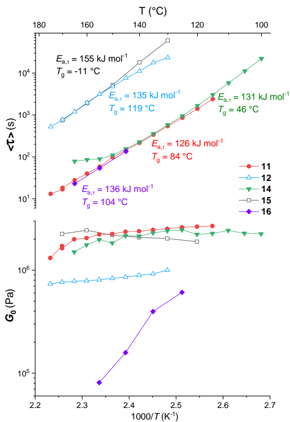
Fig. 5 Temperature dependence of top) the average relaxation times and bottom) zero-shear moduli for TPIL dynamic networks 11 (red solid circles), 12 (blue open triangles), 14 (green solid triangles). Additional data for previously reported aliphatic TPIL dynamic network 15 (black open squares) and polystyrene-based TPIL dynamic network 16 (purple solid diamonds) have been added for comparison. 21,41
