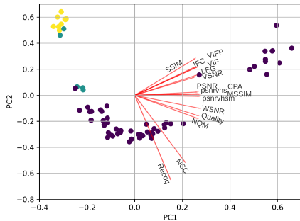
(c) j2kne
