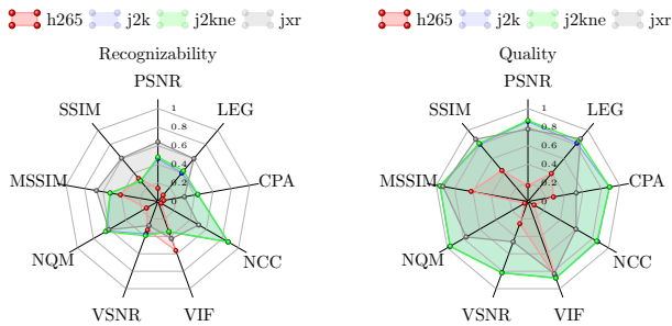
Fig. 6: Comparison of the metrics' behavior against recognizability and quality estimation tasks.
