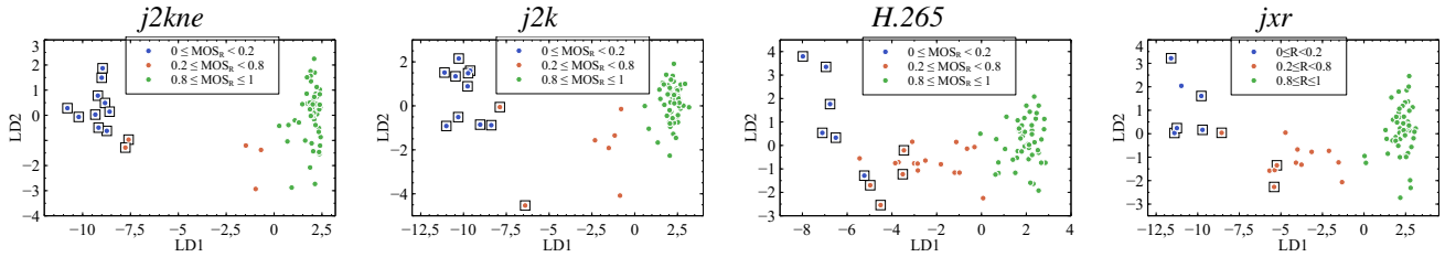
(a) Linear discriminant analysis on the given selective encryption methods.
