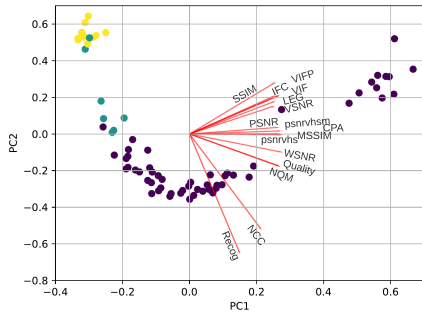
(b) j2k
