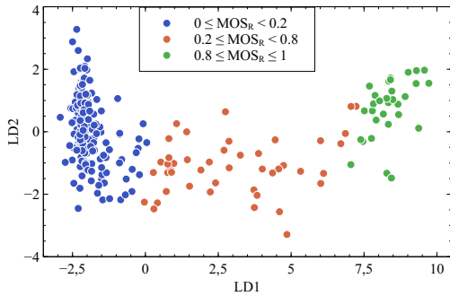
Fig. 8: LDA on the full dataset.
