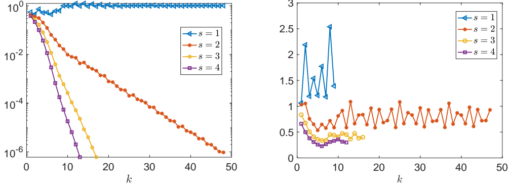
Figure 6: Relative error \frac{\|\rho_{0,s}(y_{k+1}-y_k)\|_{L^2(Q_T)}}{\|\rho_{0,s}y_k\|_{L^2(Q_T)}} (Left) and \frac{\|\rho_{0,s}(y_{k+1}-y_k)\|_{L^2(Q_T)}}{\|\rho_{0,s}(y_k-y_{k-1})\|_{L^2(Q_T)}} (Right) w.r.t. k for s \in \{1, 2, 3, 4\} .
