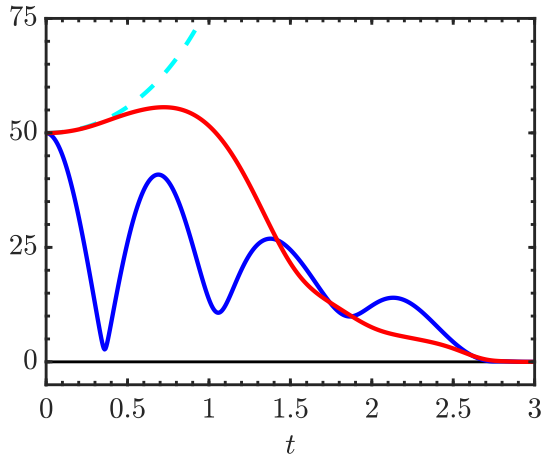
Figure 4: c_g = 10 – Evolution of \|y_4(\cdot, t)\|_{L^2(\Omega)} (—), \|y_0(\cdot, t)\|_{L^2(\Omega)} (—) and \|y(\cdot, t; 0)\|_{L^2(\Omega)} (---) w.r.t. t .
