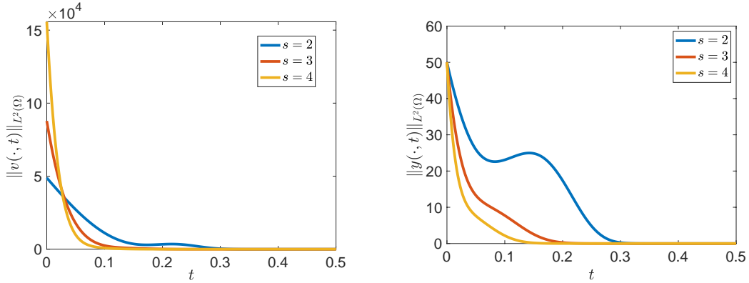
Figure 7: Evolution of \|v_{k^*}(\cdot, t)\|_{L^2(\Omega)} and \|y_{k^*}(\cdot, t)\|_{L^2(\Omega)} w.r.t. t \in [0, T] for c_{u_0} = 10 , c_f = -5 and s \in \{2, 3, 4\} .
