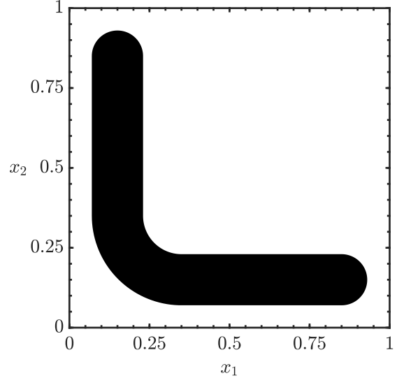
Figure 2: Control domain \omega \subset \Omega = (0, 1)^2 (black zone).
