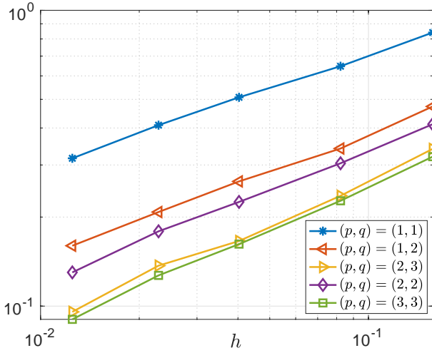
Figure 1: Relative error on the approximation of the boundary control \|\partial_\nu \phi_h(1, \cdot) - v\|_{L^2(0, T)} / \|v\|_{L^2(0, T)} with respect to h for different approximations.
