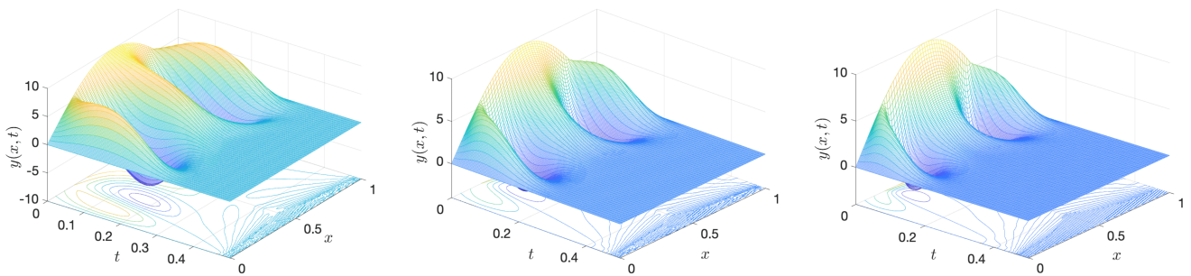
Figure 9: The controlled solution y_{k^*} in Q_T for c_{u_0} = 10 , c_f = -5 and s \in \{2, 3, 4\} .
