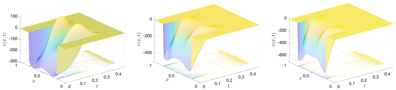
Figure 8: The control v_{k^*} in Q_T for c_{u_0} = 10 , c_f = -5 and s \in \{2, 3, 4\} .
