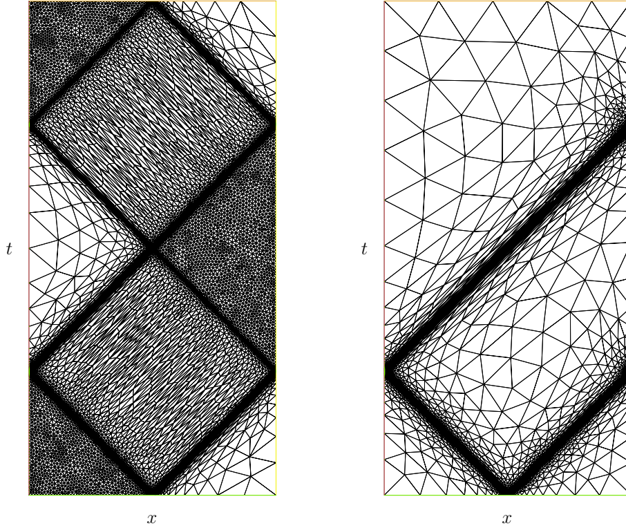
Figure 3: Locally refine spacetime meshes with respect to \phi_h (Left) and \lambda_h (Right).
