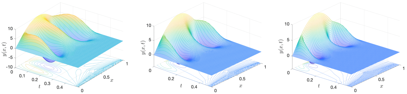
Figure 10: The controlled solution y_{k^*} in Q_T for c_{u_0} = 10 , c_f = -5 and s \in \{2, 3, 4\} .
