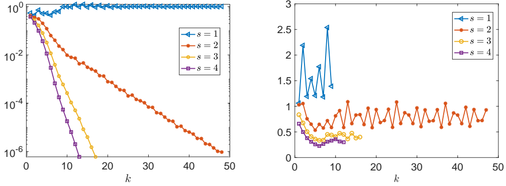
Figure 7: \frac{\|\rho_{0,s}(y_{k+1}-y_k)\|_{L^2(Q_T)}}{\|\rho_{0,s}y_k\|_{L^2(Q_T)}} (Left) and \frac{\|\rho_{0,s}(\Lambda_s(y_k)-\Lambda_s(y_{k-1}))\|_{L^2(Q_T)}}{\|\rho_{0,s}(y_k-y_{k-1})\|_{L^2(Q_T)}} (Right) w.r.t. k for s \in \{1, 2, 3, 4\} .
