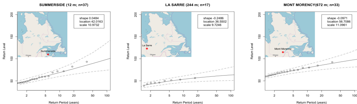
Figure 19: Locations of 3 selected stations and adequacy of fitted GEV model through the associated return level plots.
