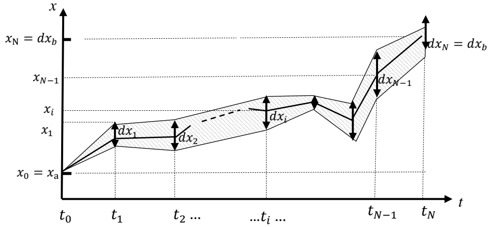
Figure 3: A 1-dimensional path of N steps along x axis from a and b , illustrated in space-time x-t . The hatched band represents the width Dx = dx_1 dx_2 \dots dx_N . The width of the path at the step at x_i is given by the tolerance dx_i . It is obvious that if one of the N tolerances dx_i is zero, the path is at once deadlocked since its width Dx = 0 .
