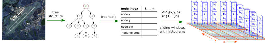
Fig. 7: Computation of fast pattern spectra consists of populating the local histograms for sliding windows. The algorithm traverses the tree structure and adds the contribution of each node to the corresponding histogram bin.
