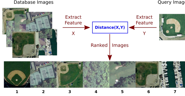
Fig. 2: General framework of content based image retrieval. The images in the database are sorted based on their distances to a query image. (The images are selected from Merced dataset [15] only for illustration. )
