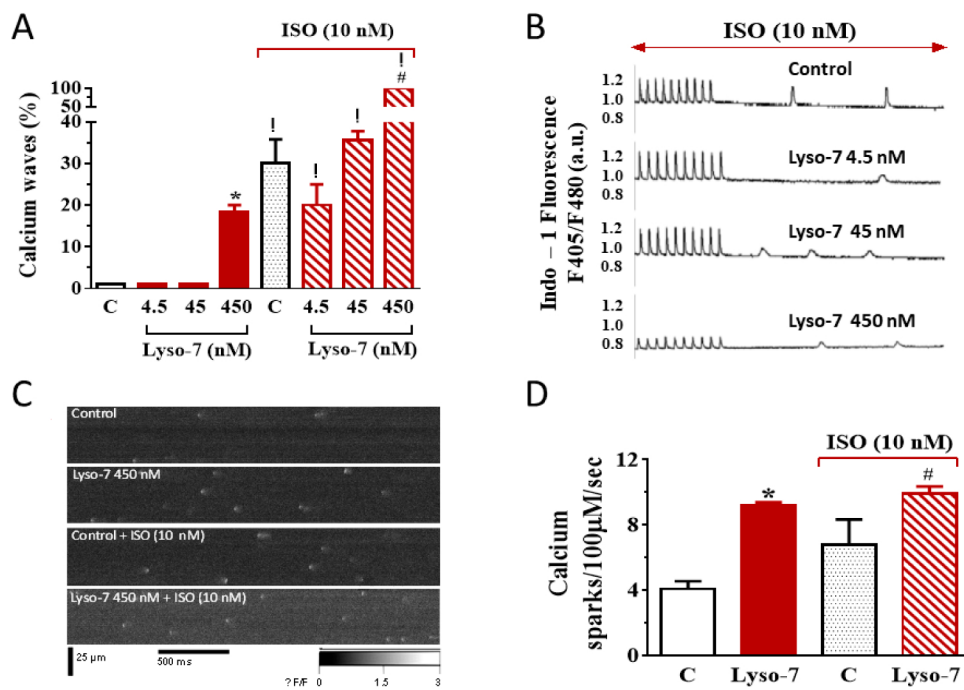
Figure 7. Acute in vitro effect of Lyso-7 on cardiomyocytes' abnormal spontaneous diastolic Ca 2+ events under Isoproterenol (ISO, 10 nM) challenge. (A) percentage of cardiomyocytes developing at least one spontaneous Ca 2+ wave in the absence (left panel) and presence (right panel) of Isoproterenol (ISO, 10 nM) during resting periods after a train of field stimulation at 1 Hz in cardiomyocytes. (B) Representative recordings of Ca 2+ waves under ISO. n = 12–18 cells. (C) Typical line-scan confocal images of Ca 2+ sparks from Fluo-4-AM loaded cardiomyocytes; n = 7–10. (D) Mean of frequency of Ca 2+ sparks measured in the different conditions indicated. C = Control refers to the absence of Lyso-7 (450 nM). We used a t -test. p < 0.05, * Lyso-7 vs. Control in the absence of ISO (left part of the panel); # Lyso-7 vs. Control in the presence of ISO (right part of the panel); ! with ISO vs. without ISO.
