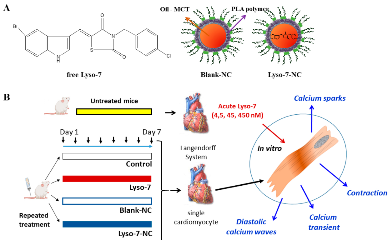
Figure 1. Chemical structure of Lyso-7 and schematic representation of polymeric nanocapsules (A). Presentation of the experimental protocol used to treat mice and isolate the cardiomyocytes to test cardiotoxicity of the formulations (B) directly in vitro (acute effects) or after in vivo treatment followed by cardiomyocyte isolation.
