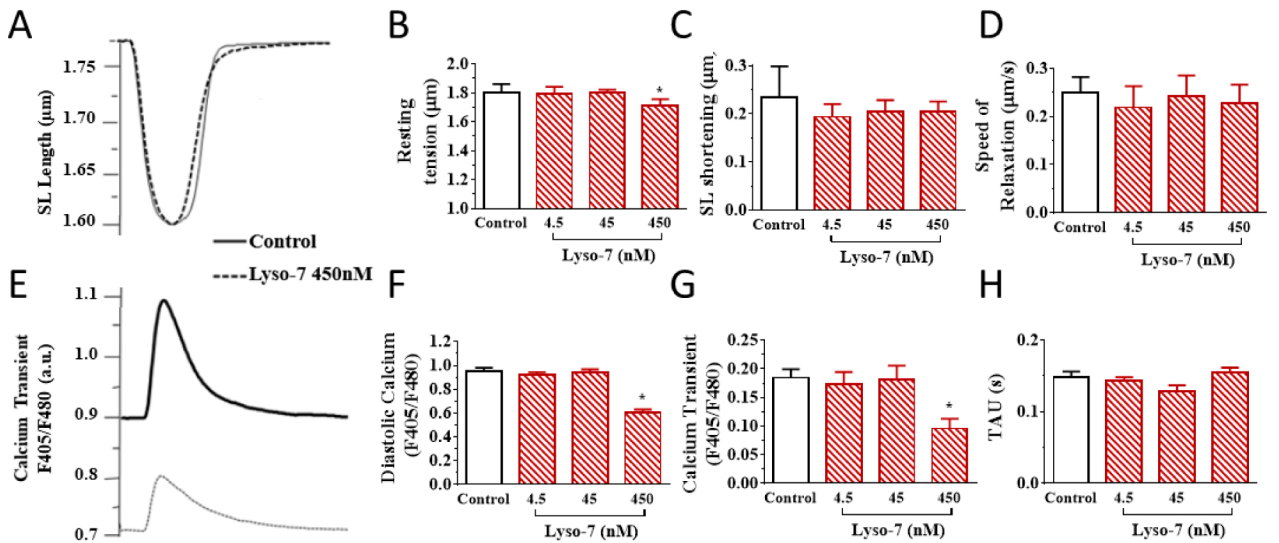
Figure 6. Acute in vitro effect of Lyso-7 on contraction (A–D) and \text{Ca}^{2+} transient (E–H) of cardiomyocytes under IsoproTable 10. nM). Typical recordings of Lyso-7 (450 nM) effects on (A) sarcomere length (SL) shortening and (E) \text{Ca}^{2+} transient, both under field stimulation at 1 Hz. (B–D) averaged data of resting SL, SL shortening and relaxation, respectively, and (F–H) averaged data of diastolic \text{Ca}^{2+} , \text{Ca}^{2+} transient and decay of \text{Ca}^{2+} transient (Tau), respectively, for Control, and increasing concentration of Lyso-7 (4.5, 45, and 450 nM). ANOVA followed by Tukey post-test ( p < 0.05 ). * Lyso-7 vs. Control. Control refers to the absence of Lyso-7. n = 12 –18.
