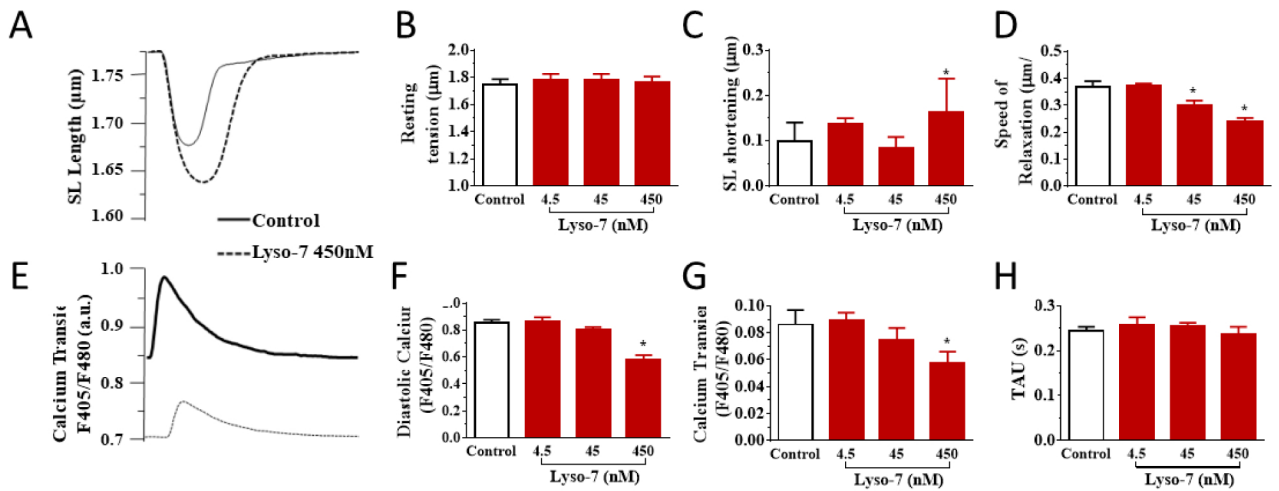
Figure 5. Acute effect of Lyso-7 on contraction (A–D) and \text{Ca}^{2+} transient (E–H) in cardiomyocytes of untreated mice. Typical recordings of Lyso-7 (450 nM) effects on sarcomere length (SL) shortening (A) and \text{Ca}^{2+} transient (E), both under field stimulation at 1 Hz. (B–D) averaged data of resting SL, SL shortening and relaxation, respectively, and (F–H): averaged data of diastolic \text{Ca}^{2+} , \text{Ca}^{2+} transient and decay of \text{Ca}^{2+} transient (Tau), respectively, for Control, and increasing concentration of Lyso-7 (4.5, 45, and 450 nM). ANOVA followed by Tukey post-test ( p < 0.05 ). * Lyso-7 vs. Control. Control refers to the absence of Lyso-7. n = 12 –18.
