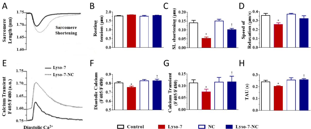
Figure 2. Effect of in vivo administration of Lyso-7 and Lyso-7-NC (1.6 mg/kg, once a day for seven days) on contraction (A–D) and \text{Ca}^{2+} transient (E–H) in freshly isolated cardiomyocytes. Typical recordings of the effects of Lyso-7 (free form) and Lyso-7-NC on sarcomere length (SL) shortening (A) and \text{Ca}^{2+} transient (E), both under field stimulation at 1 Hz. (B–D): averaged data of resting SL, SL shortening and relaxation, respectively, and (F–H): averaged data of diastolic \text{Ca}^{2+} , \text{Ca}^{2+} transient and decay of \text{Ca}^{2+} transient (Tau), respectively, all for the four experimental groups (Control, Lyso-7, NC, and Lyso-7-NC). ANOVA followed by Tukey post-test ( p < 0.05 ). * Lyso-7 vs. Control; ! Lyso-7-NC vs. Lyso-7. n = 4 ; n = 12-18 .
