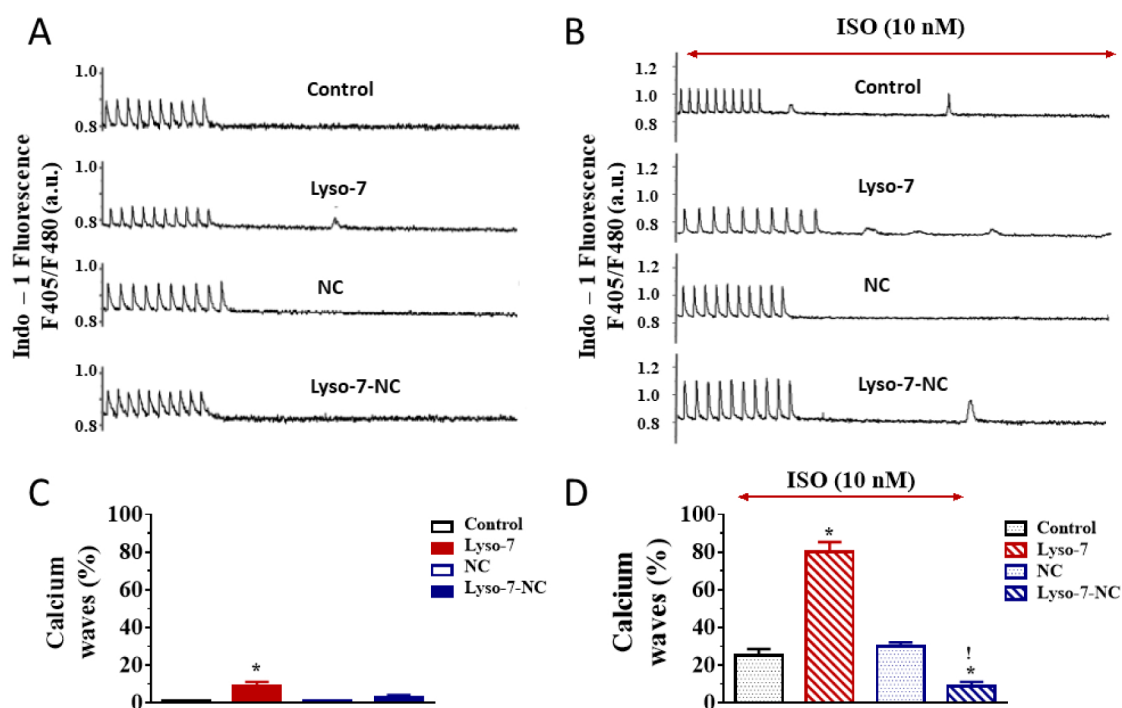
Figure 4. Effect of in vivo administration of Lyso-7 and Lyso-7-NC (1.6 mg/kg, once a day for seven days) on cardiomyocytes' ectopic diastolic \text{Ca}^{2+} waves. (A) Representative recordings of \text{Ca}^{2+} waves during resting periods after a train of field stimulation at 1 Hz in cardiomyocytes from the four experimental groups (Control, Lyso-7, NC, and Lyso-7-NC); (B) Representative recordings of \text{Ca}^{2+} waves during resting periods after a train of field stimulation at 1 Hz in cardiomyocytes from the four the same experimental groups treated in vitro with Isoproterenol (ISO, 10 nM); (C,D) percentage of cardiomyocytes developing at least one spontaneous \text{Ca}^{2+} wave in absence and presence of ISO (10 nM) in vitro, respectively, for the four experimental groups (Control, Lyso-7, NC, and Lyso-7-NC). We used a t -test. p < 0.05 , * Lyso-7 vs. control; ! Lyso-7-NC vs. Lyso-7. a.u.: arbitrary units. n = 4 ; n = 12-18 .
