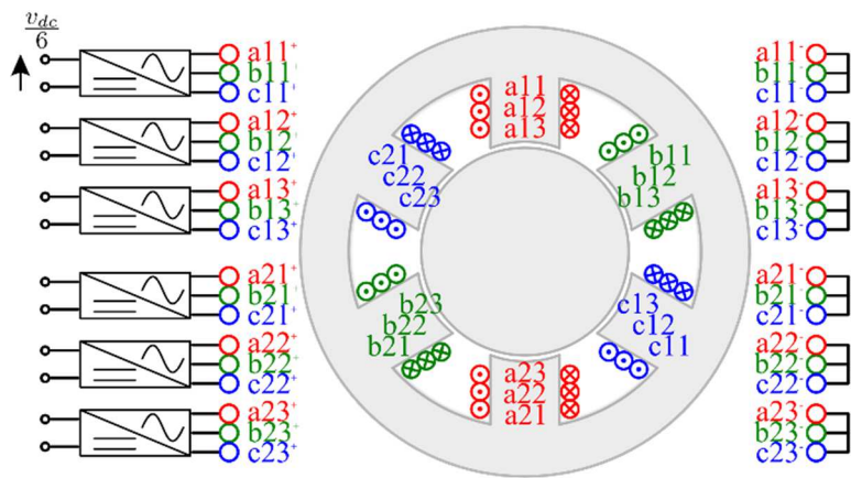
c) Split by bundle of turns: 3-phase machine (18 sub-windings, several of them on the same tooth) fed by 6 independent 3-phase converters
