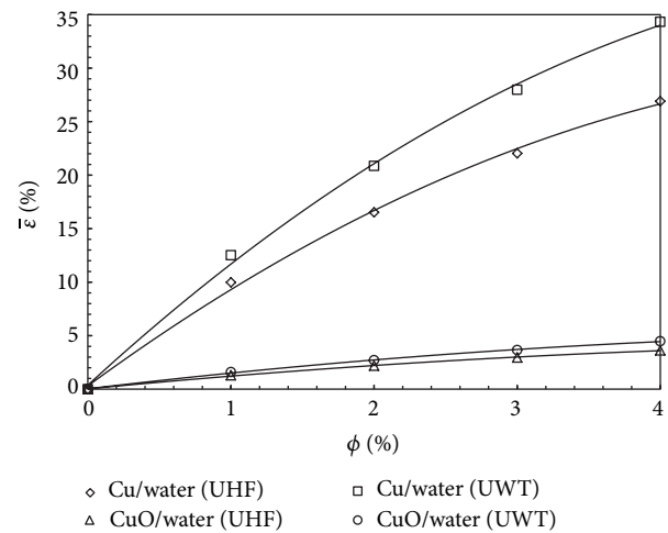
FIGURE 6: Average heat transfer performance versus the particle volume fraction.
