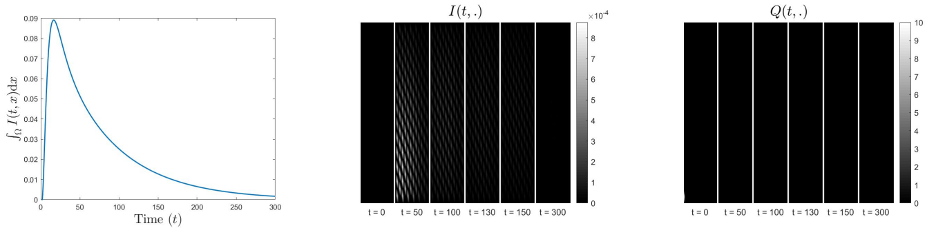
Figure 2: Asymptomatic extinction of the disease and convergence to the disease-free equilibrium when \mathcal{R}_0 < 1 . For I and Q dynamics, the whole domain \Omega is illustrated at different times t = 0, 50, 100, 130, 150, 300 .
