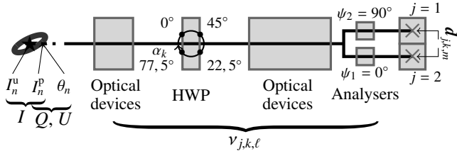
Fig. 1. Schematic view of the instrument ESO/VLT-SPHERE IRDIS showing the various optical parts that can induce polarization effects. The same notations as in the text are used (e.g., n is the pixel index in the restored maps, k is the sequence index, and j is the polarizer index of the analyzer set).
