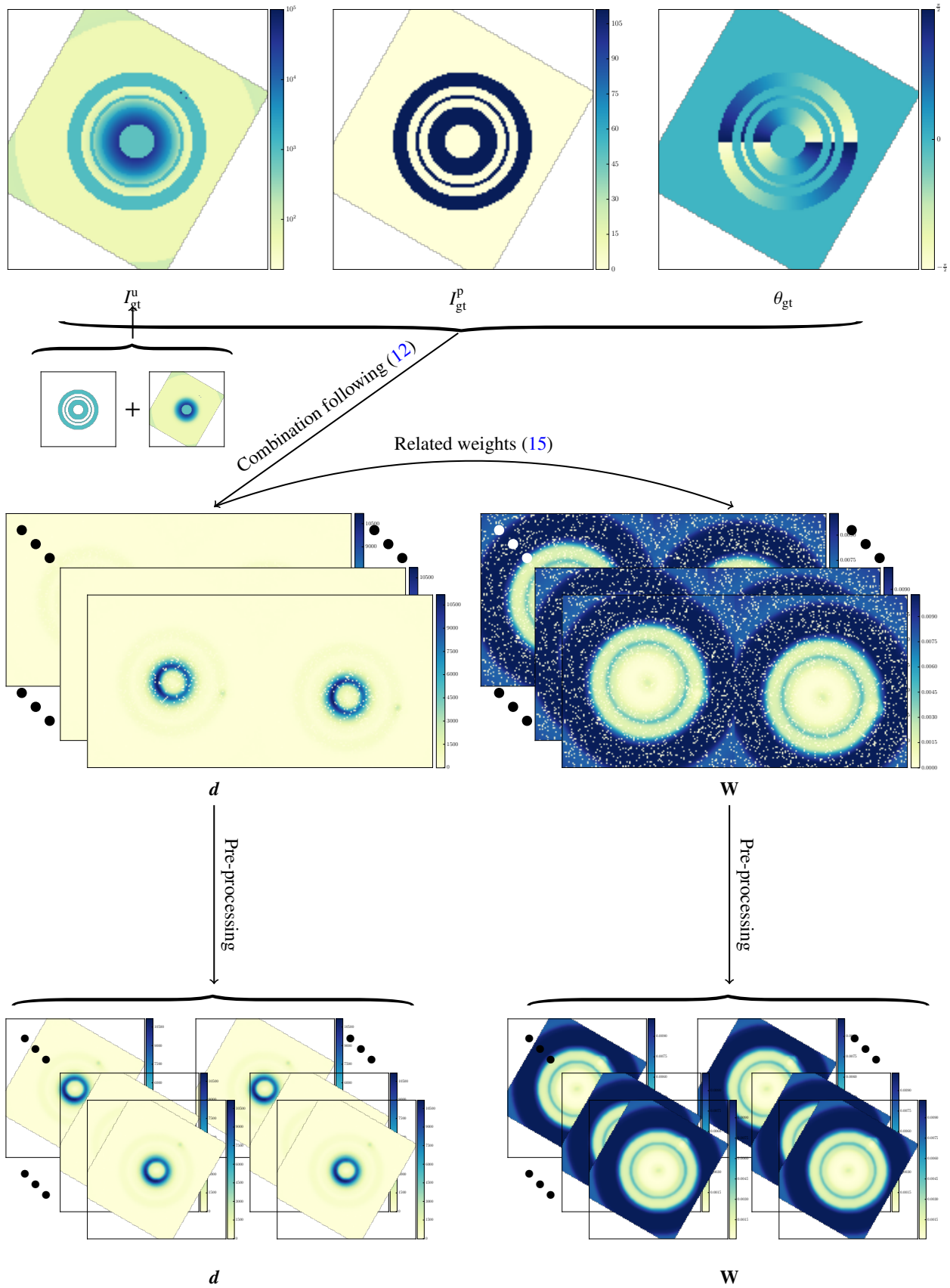
Fig. A.2. Schematic illustration describing the process of the data simulation. Starting from synthetic maps I_{\text{gt}}^u , I_{\text{gt}}^p , and \theta_{\text{gt}} based on a disc model, we generate artificial calibrated and pre-processed datasets d and associated weights W , illustrated here for \tau^{\text{disk}} = 10\% .
