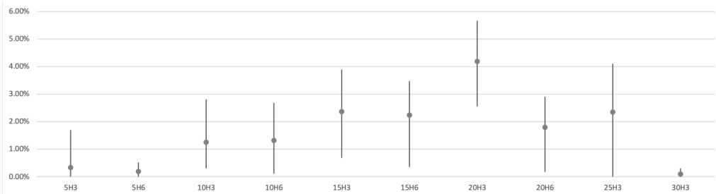
(c) |\mathcal{M}| = 60
