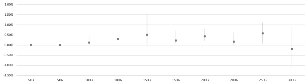
(b) |\mathcal{M}| = 30
