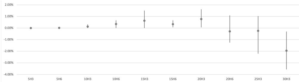
(c) |\mathcal{M}| = 60
