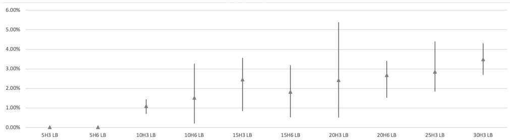
(b) |\mathcal{M}| = 30
