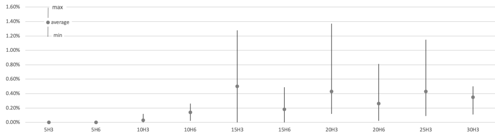
(a) |\mathcal{M}| = 12
