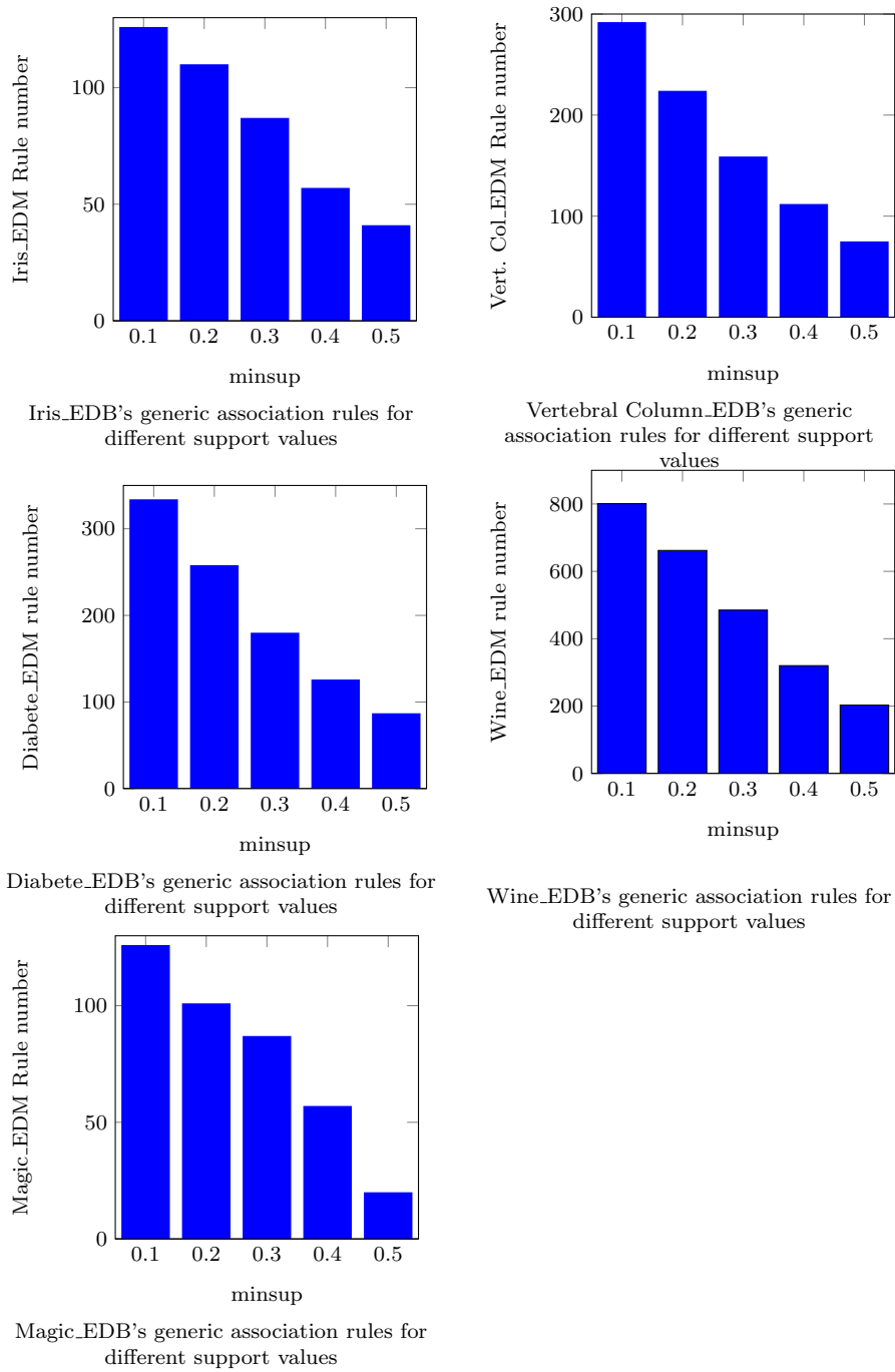
Fig. 2: Generic association rule's number for different support values
