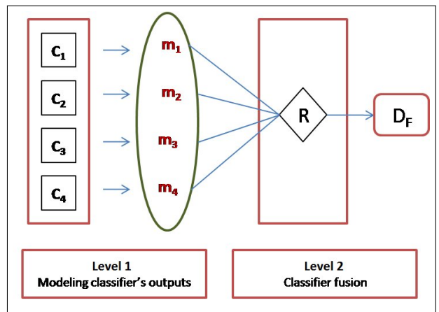
Fig. 1 Classifier fusion within the belief function framework
