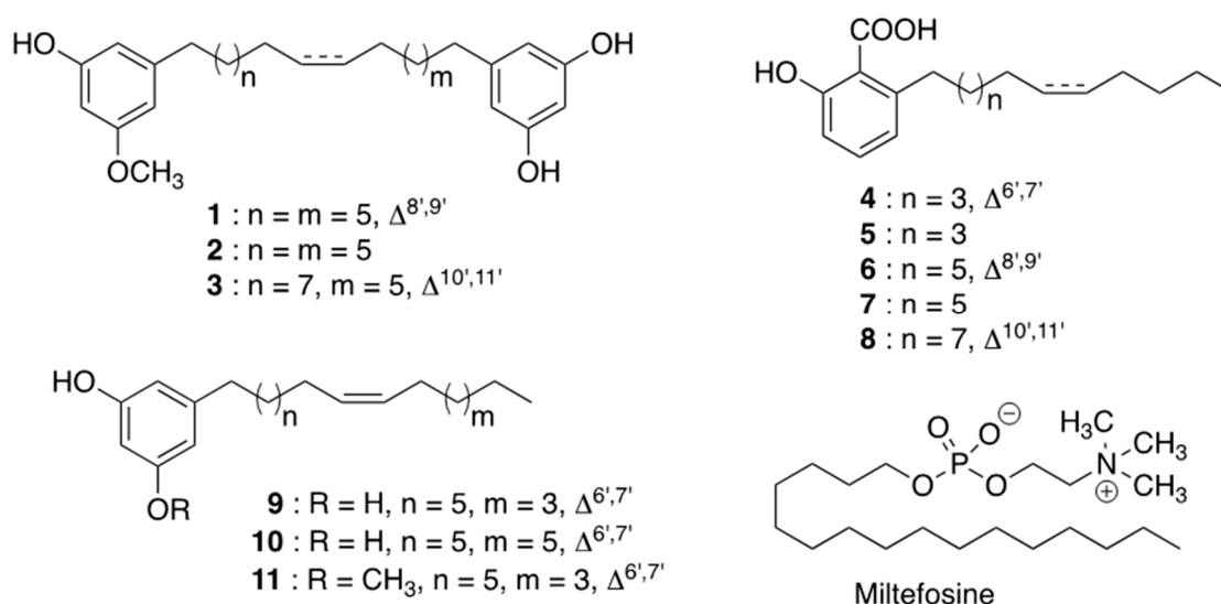
Figure 1. Structures of compounds 1–11.
