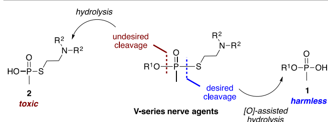
Fig. 1. General decomposition paths of V-series OPNA: VX (R 1 = Et, R 2 = i -Pr), R-VX (R 1 = i -Bu, R 2 = Et) and C-VX (R 1 = n -Bu, R 2 = Et).
