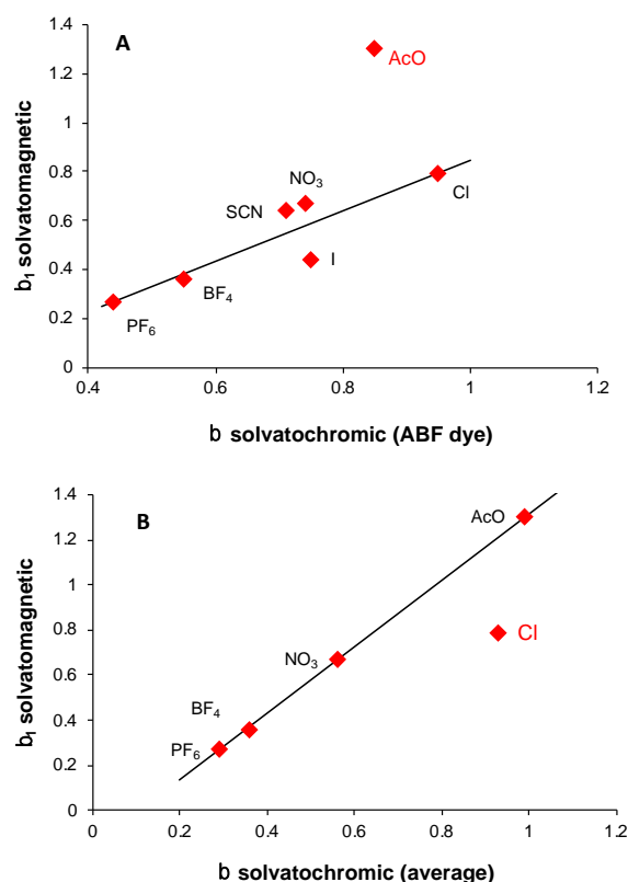
Figure 7. Comparison between the solvatomagnetic \beta_1 values of [\text{C}_4\text{mim}]\text{X} ILs and (A) the solvatochromic \beta scale based on the ABF dye (the regression line does not take into account the acetate), and (B) an averaged solvatochromic \beta scale (the regression line does not take into account the chloride).
