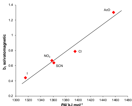
Figure 6. Correlation between the solvatomagnetic \beta_1 values of [\text{C}_4\text{mim}]\text{X} ILs and the proton affinity PA of their anion.
