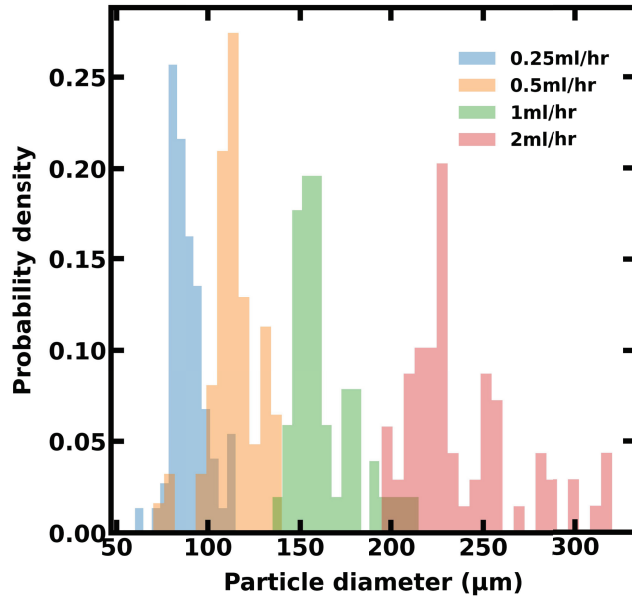
FIG. 3. Number particle size distribution measured for 4 PDMS flow rates. The glycerin flow rate is fixed to 130 \text{ mL/h} .
