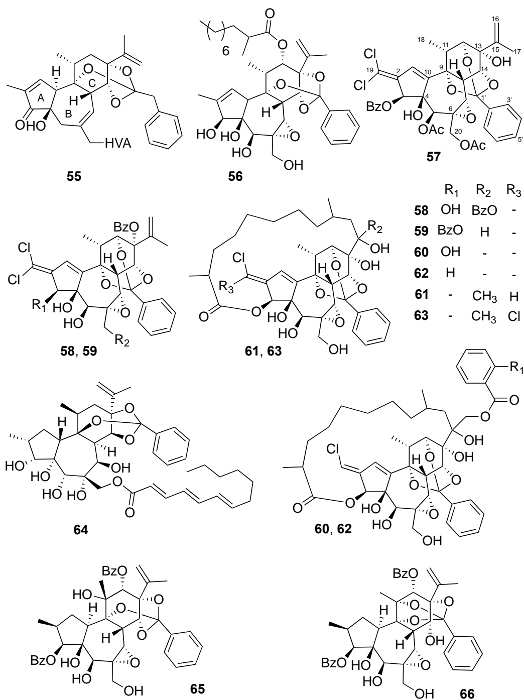
Figure 3. Structures of daphanes 55–66.
