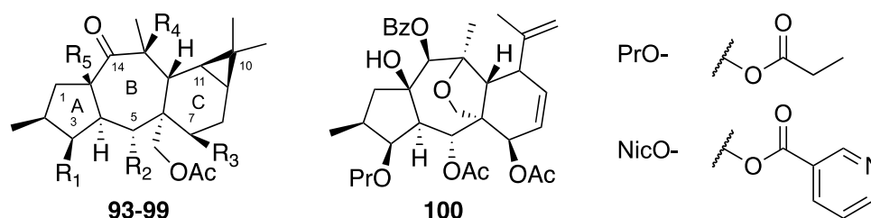
Figure 5. Structures of premyrsinanes 93–99 and myrsinane 100 .
