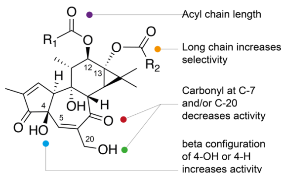
Figure 2. Structure–activity relationships of tiglianes.
