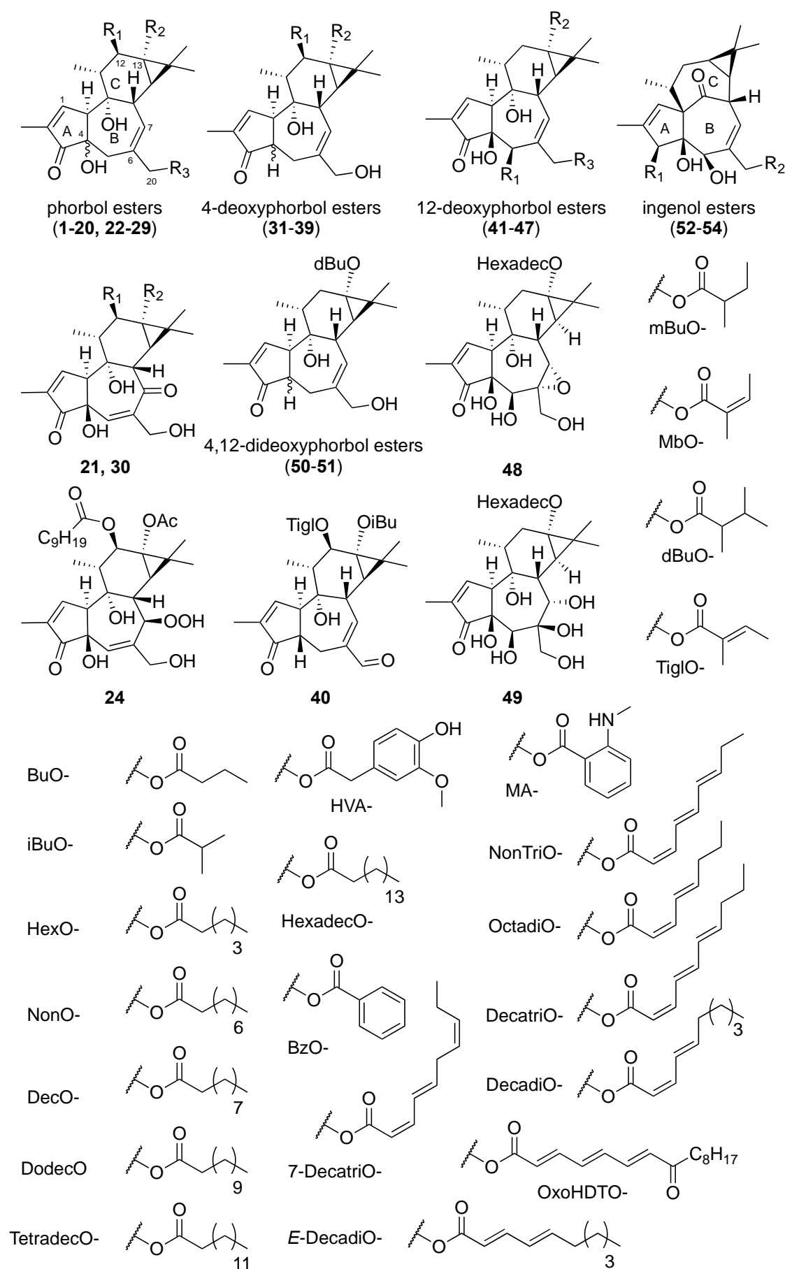
Figure 1. Structures of tiglianes 1–51 and ingenanes 52–54.
