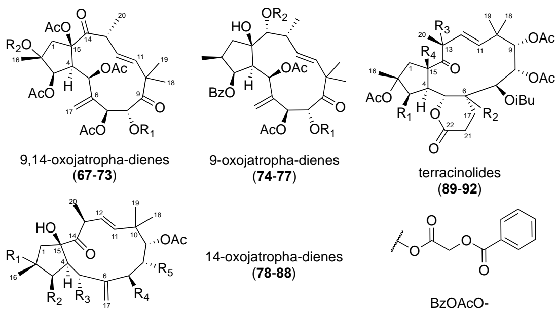
Figure 4. Structures of jatrophanes 67–92.
