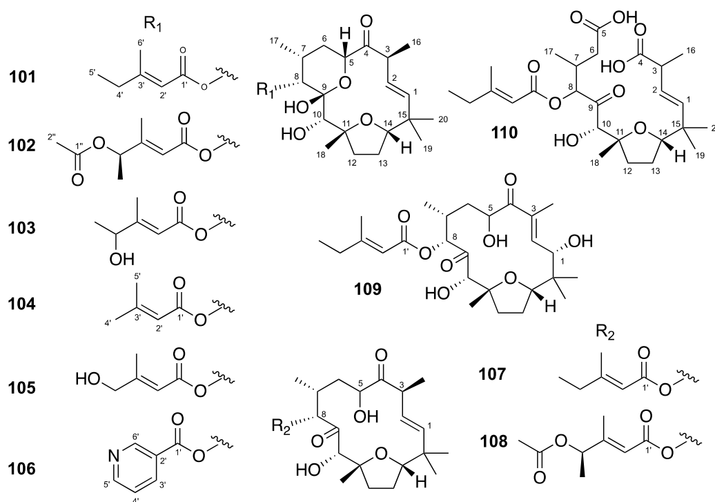
Figure 6. Structures of flexibilanes 101–110.
