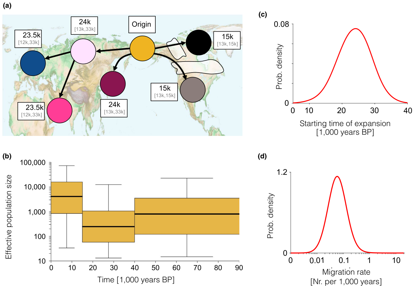
FIGURE 5 The inferred scenario of wolf demography from the Bayesian analysis using our spatially and temporally explicit model (see Figure 4 and the main text). (a) Geographical representation of the expansion scenario (out of Beringia) with median and 95% confidence interval (CI) for the date of the population replacement in each deme given in white boxes next to each deme. (b) Effective population size (thick line, boxes and whiskers show the median, interquartile range and 95% CI, respectively, for each time period). (c) Posterior distribution of migration rate and (d) starting time of expansion [Colour figure can be viewed at wileyonlinelibrary.com ]
