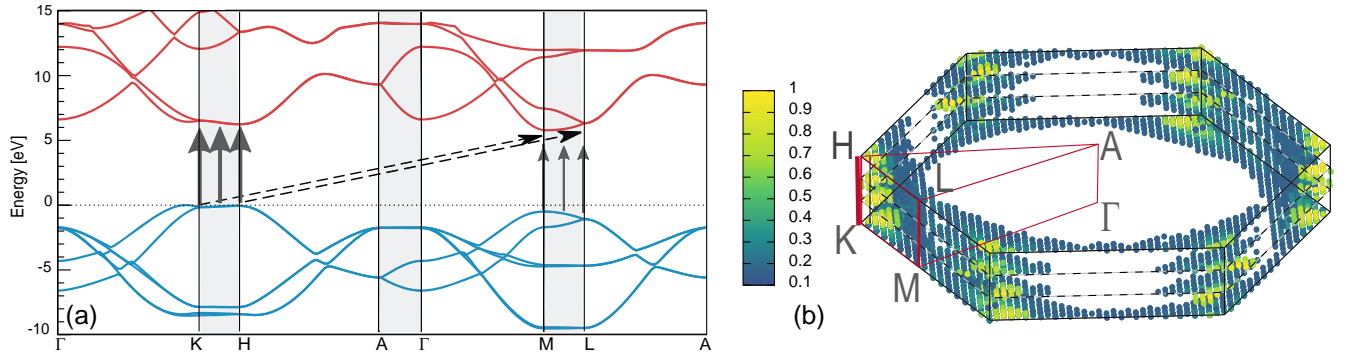
FIG. 1. (a) Electronic band structure evaluated in the framework of many-body GW calculations. The shaded areas indicate the paths that are parallel to the c -axis in the Brillouin zone of bulk hBN. Arrows in dark gray (dashed black) indicate the parallel direct (indirect) transitions contributing to the formation of the direct ( dX ) and indirect ( iX ) excitons, respectively. (b) Color map in the Brillouin zone of bulk hBN of the weighted oscillator strengths A_{\lambda}^t \rho^t(\mathbf{q}) [as defined in Eq. (1)] building the dX exciton. For the sake of clarity, the map is limited to the points of the prevailing direct independent-particle transitions t , that contribute in total to 80% of the dX absorption. The irreducible part of the Brillouin zone is delimited by red lines, which are thicker for the KH and ML paths.
