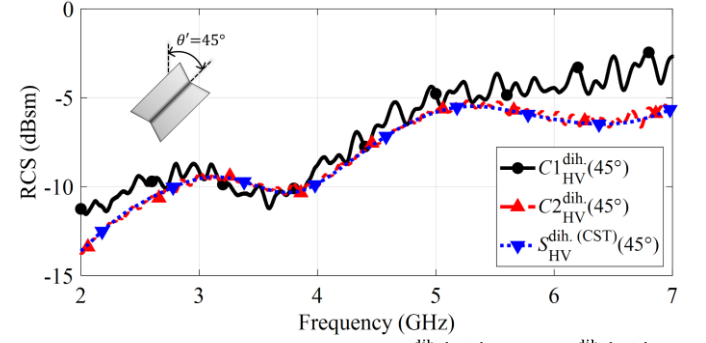
Fig. 10 The calibrated RCS signals C1_{HV}^{\text{dih}}(45^\circ) and C2_{HV}^{\text{dih}}(45^\circ) in comparison to the CST estimated signal S_{HV}^{\text{dih}}(\text{CST})(45^\circ) for the dihedral tilted at 45^\circ as the test target.
