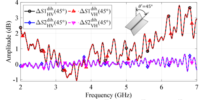
Fig. 11. Calibration error signals \Delta S1_{HV}^{\text{dih}}(45^\circ) , \Delta S1_{VH}^{\text{dih}}(45^\circ) , \Delta S2_{HV}^{\text{dih}}(45^\circ) , and \Delta S2_{VH}^{\text{dih}}(45^\circ) for the dihedral tilted at 45^\circ as the test target.
