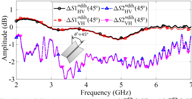
Fig. 17 Calibration error signals \Delta S1_{HV}''dih(45^\circ) , \Delta S1_{VH}''dih(45^\circ) , \Delta S2_{HV}''dih(45^\circ) and \Delta S2_{VH}''dih(45^\circ) for the dihedral tilted at 45^\circ as the test target.
