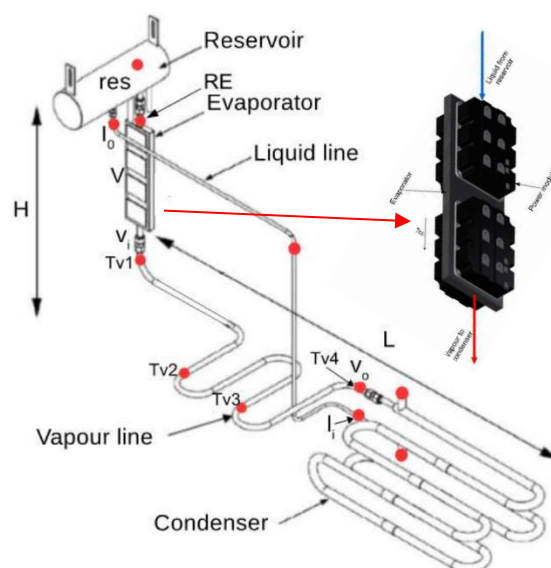
Fig. 4: Concept scheme of a CPLIP and power electronics module/evaporator assembly [2]
