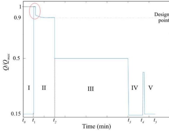
Fig. 1: Example of power electronic converter total thermal losses as function of time during a flight mission profile [2]
