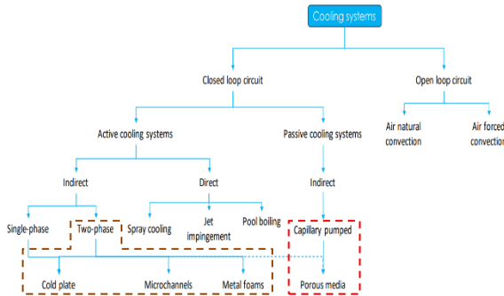
Fig. 2: Cooling systems classification [3]
