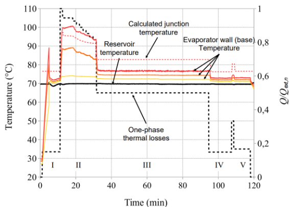
Fig. 5: Experimental response of a single-evaporator CPLIP to a one-phase thermal losses mission profile corresponding to Fig. 1 [2]
