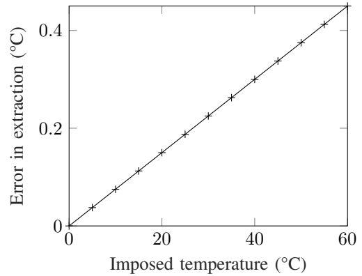
Fig. 5. Error between the extracted temperature using (11) and the simulated temperature when the approximation K=1 is used.
