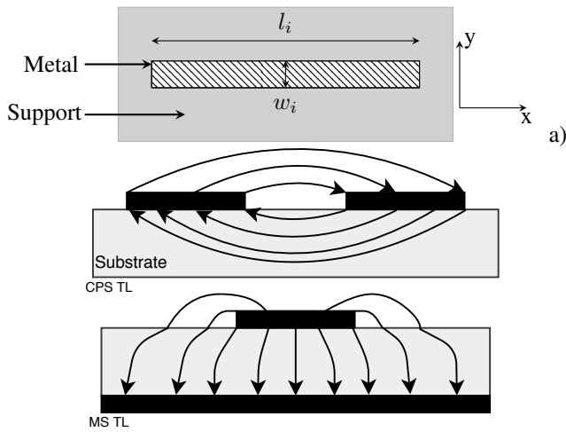
Fig. 17. (a) Resonant scatterer-based microstrip TL. Below the dielectric support of height h a ground plane is placed. Nominal dimension are w=2\text{mm} , l_1=2.5\text{cm} , l_2=2.2\text{cm} and l_3=2\text{cm} for the three resonators respectively. The polarisation of the electric field used to excite the resonator is along x . (b) Electric field configuration for the two different TL resonators.
