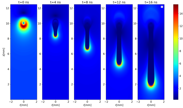
Figure 7: (colored) Simulation 2 . Evolution of the electric field strength |\mathbf{E}| ( MVm^{-1} ) of a downward propagation of the streamer. Results are obtained by SGCC_2^{3,0} . Although the domain stretches to r = 1.25cm , visualization is only shown up to r = 2mm .
