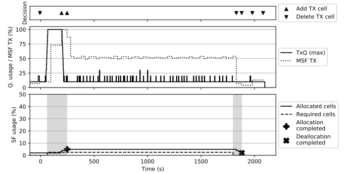
Figure 7. Evolution of allocated cells with time on node 2 with a generated traffic load of 0.5 pkts/sf/node. Allocation/deallocation periods are shaded in grey.
