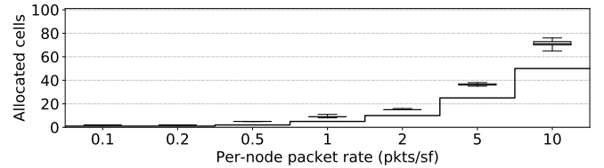
Figure 10. Number of cells allocated on node 2, as a function of per-node packet rate.
