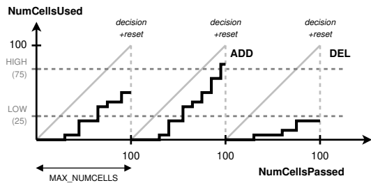
Figure 4. Decision to request/delete cells, with hysteresis.
