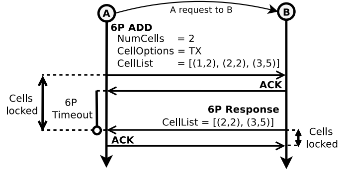
Figure 3. An example of a 2-step 6top ADD transaction. The request is made from node A to node B. Node A requests two cells among three proposed candidates. Node B responds with two selected cells among the candidates.
