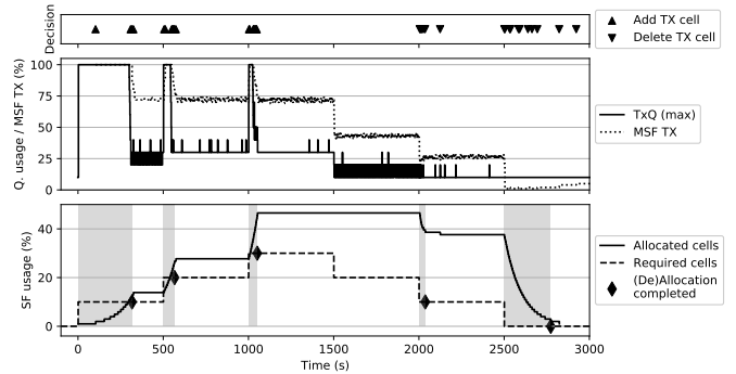
Figure 11. Evolution of allocated cells along time with a traffic load varying in the 0 – 30 pkt/sf range with rate change steps of 10 pkt/sf each. Allocation/deallocation periods are shaded in gray.
