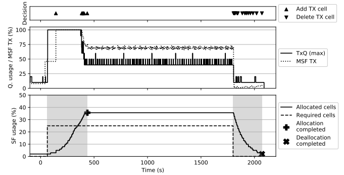
Figure 8. Evolution of allocated cells with time on node 2 with a generated traffic load of 5 pkts/sf/node. Allocation/deallocation periods are shaded in grey.
