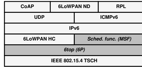
Figure 2. Network stack in the 6TiSCH architecture.
