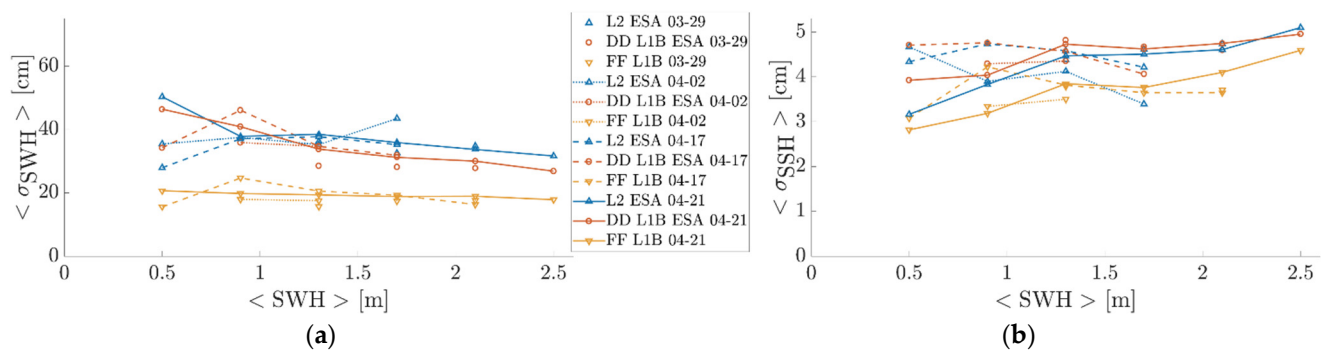
Figure 5. The precision of the selected retrieved geophysical parameters from different tracks, measured as the mean of the 20-Hz standard deviations, as a function of averaged SWH, \langle \text{SWH} \rangle : (a) The precision of the retrieved SWH, denoted by \langle \sigma_{\text{SWH}} \rangle ; (b) The precision of the retrieved Sea Surface Height (SSH), denoted by \langle \sigma_{\text{SSH}} \rangle .
