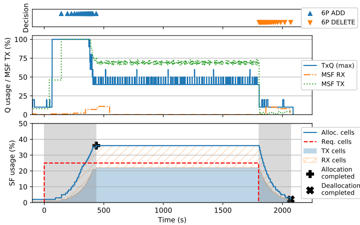
Fig. 9: Evolution of allocated cells with time on node 2 with a generated traffic load of 5 pkts/sf/node. Allocation/deallocation periods are shaded in gray.
