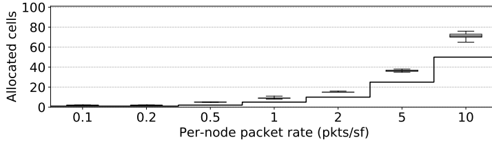
Fig. 10: Number of cells allocated on node 2, as a function of per-node packet rate. The boxes represent the amount of cells allocated across multiple runs of the same simulation. The black line represents the minimum amount of cells, N_{\text{req}} , required to transport the CBR traffic.
