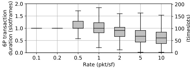
Fig. 19: Duration of 6P transactions (excluding outliers).
