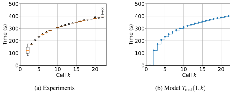
Fig. 17: MSF convergence time for static traffic 5 pkts/sf, observed on node 2.
