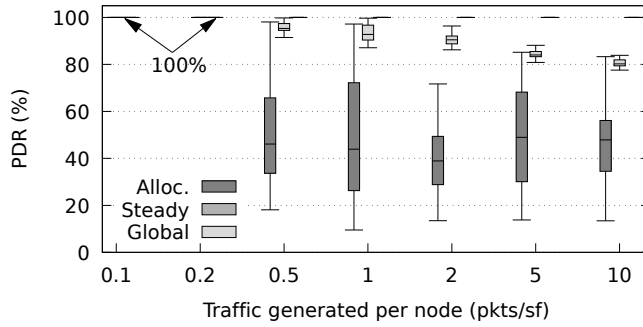
Fig. 20: Comparison of end-to-end PDR during different periods of the simulation.
