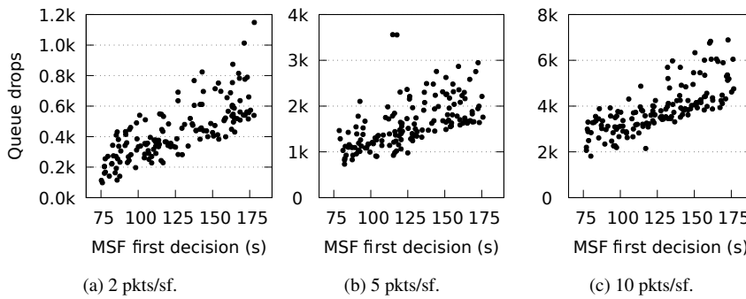
Fig. 23: Correlation between the occurrence of MSF's first decision and the number of queue overflow drops. The time to MSF's first decision can vary significantly from one run to another, delaying resource allocation and resulting in more packet losses.
