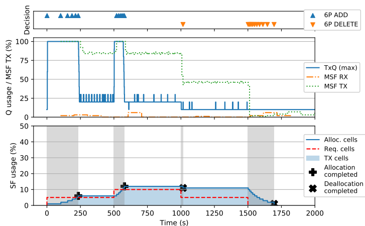
(a) Thresholds of 45% and 95%.
