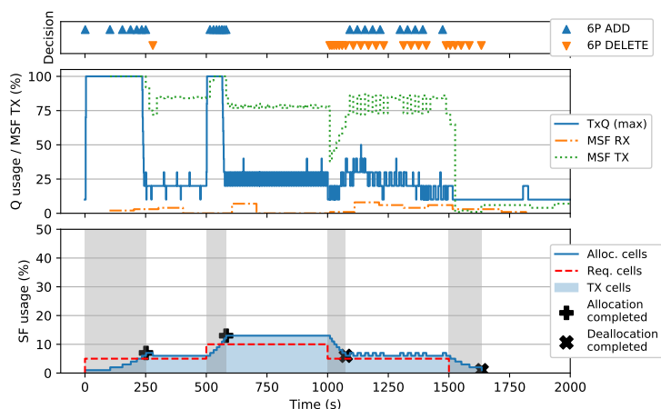
(b) Thresholds of 75% and 85%.
