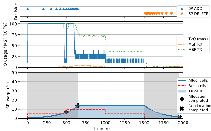
(c) MAX\_NUMCELLS = 200 .
