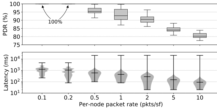
Fig. 6: End-to-end PDR and latency for the application packets carried by node 2. Whiskers on the figures represent the minimum and maximum values, the middle horizontal line the median. In the PDR figure, the intermediate box lines represent the 25th and 75th percentiles.
