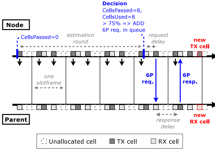
Fig. 13: Duration of a single MSF allocation: traffic estimation, decision to allocate and 6P transaction.
