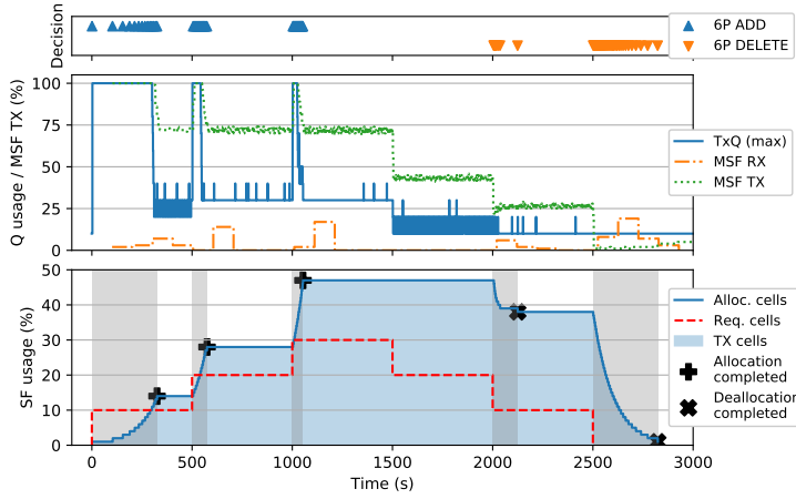
Fig. 11: Evolution of allocated cells along time with a traffic load varying in the 0 – 30 pkt/sf range with rate change steps of 10 pkt/sf each. Allocation/deallocation periods are shaded in gray.
