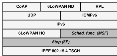
Fig. 2: Network stack in the 6TiSCH architecture.
