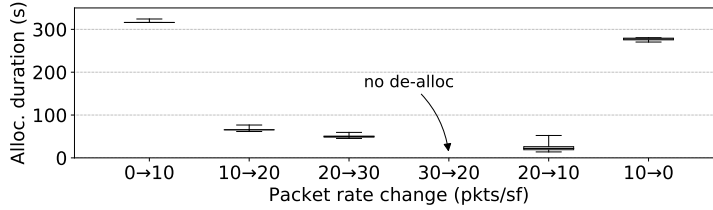
Fig. 12: Duration for MSF to reach a stable state and allocate all necessary cells after a change in traffic rate.
