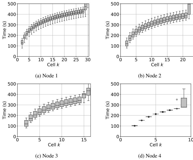
Fig. 14: Time between application start and decision to allocate cell k . Each boxplot summarizes the distribution of this time across the 50 runs for a specific cell k . The y-axis is cut at 500 s although there are a few higher values for the latest cell allocations.
