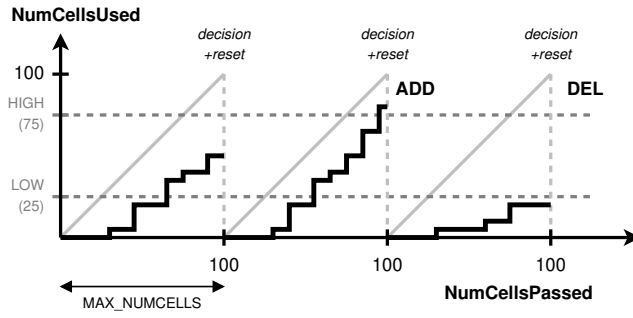
Fig. 4: Decision to request/delete cells, with hysteresis.
