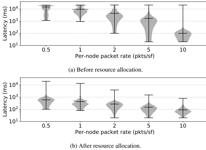
Fig. 7: Latency for the application packets carried by node 2 before and after allocating the necessary resources. Whiskers on the figures represent the minimum and maximum values, the middle horizontal line the median.
