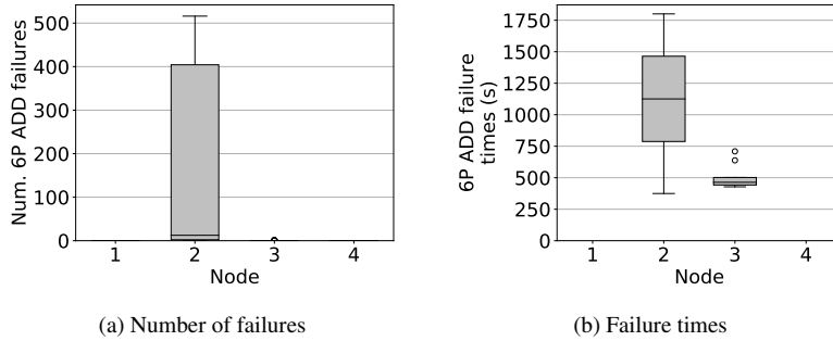
Fig. 22: 6P ADD failures at rate 10 pkts/sf. Fig. 22a shows the number of 6P ADD requests initiated by each node that resulted in a failure because the parent slotframe is full and thus cannot fulfill the request. Fig. 22b shows, with the same failures, the time required by each node to complete the 6P ADD transactions and have the cells allocated in its slotframe.
