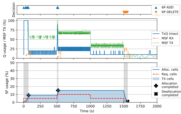
(a) MAX\_NUMCELLS = 25 .
