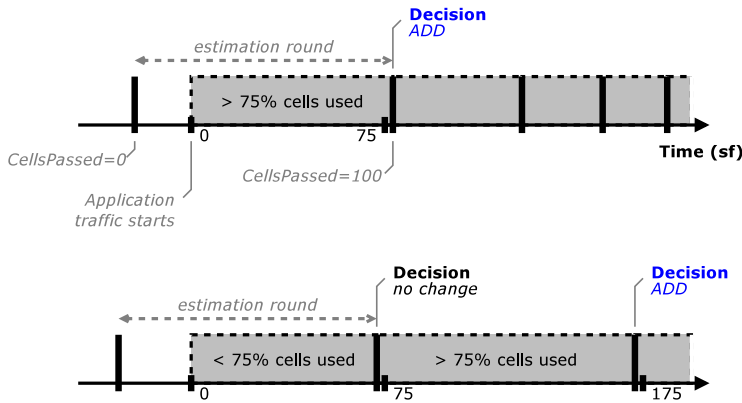
Fig. 15: Variance in the occurrence of MSF's first decision.
