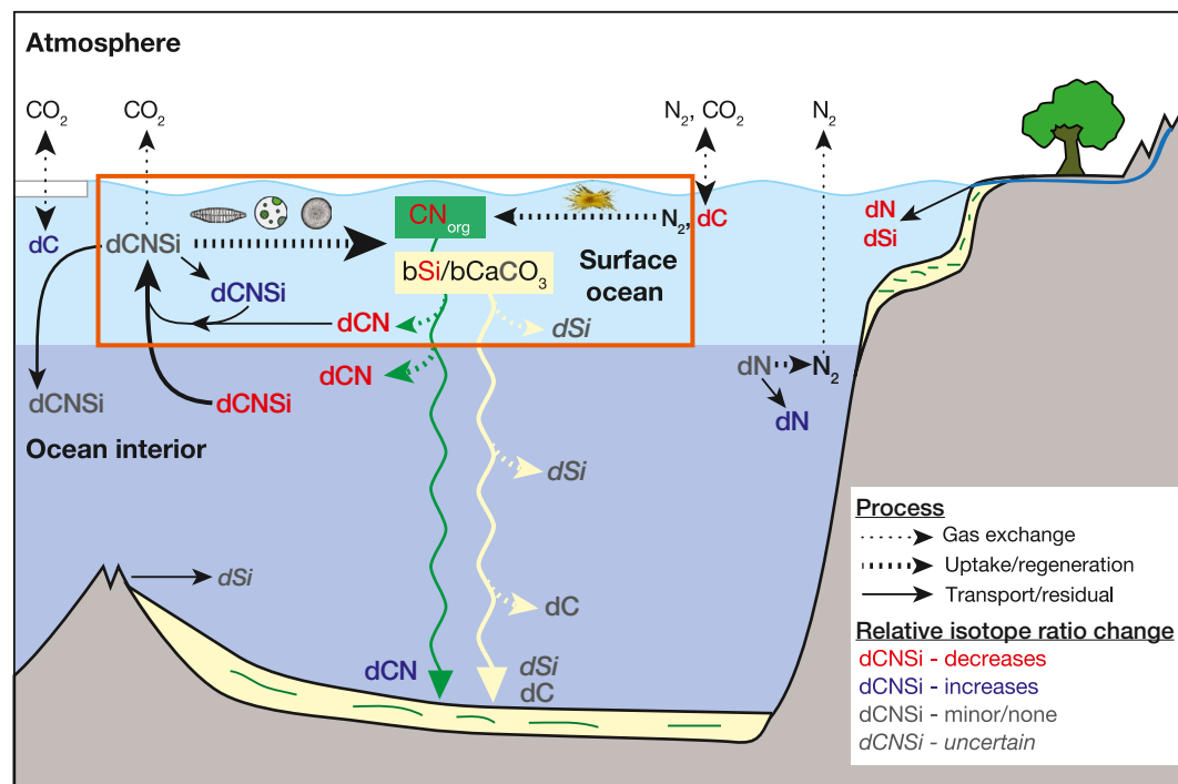
Figure 1. Schematic summary of processes affecting the isotopic composition of dissolved C, N, and Si (dCNSi). Processes related to biological productivity are outlined in the orange box. Gas exchange processes are indicated by dotted arrows; uptake and regeneration follow dashed arrows. Solid arrows indicate dissolved element transport due to ocean circulation or sinking, or the residual dissolved element pool resulting from incomplete consumption during uptake. Red/blue/gray/italicized elements denote a relative decrease/increase/minor/uncertain change to the isotopic composition ( \delta -value) of the element resulting from the associated process. Basemap modified after Hain et al. (2014).
