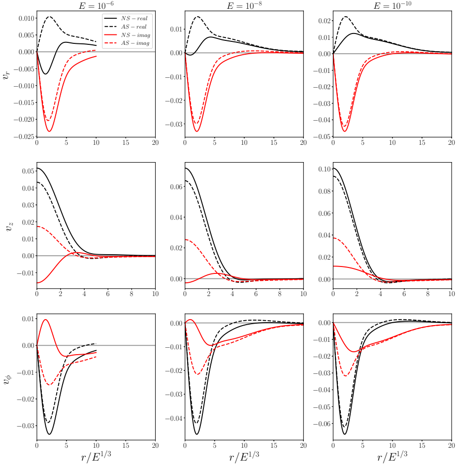
FIGURE 14. Comparison of asymptotic solutions and numerical results of three velocity components on the line perpendicular to the axis at the reflection point (0, \eta / \cos \theta_c) for three Ekman numbers.
