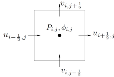
FIGURE 4. Staggered grid
