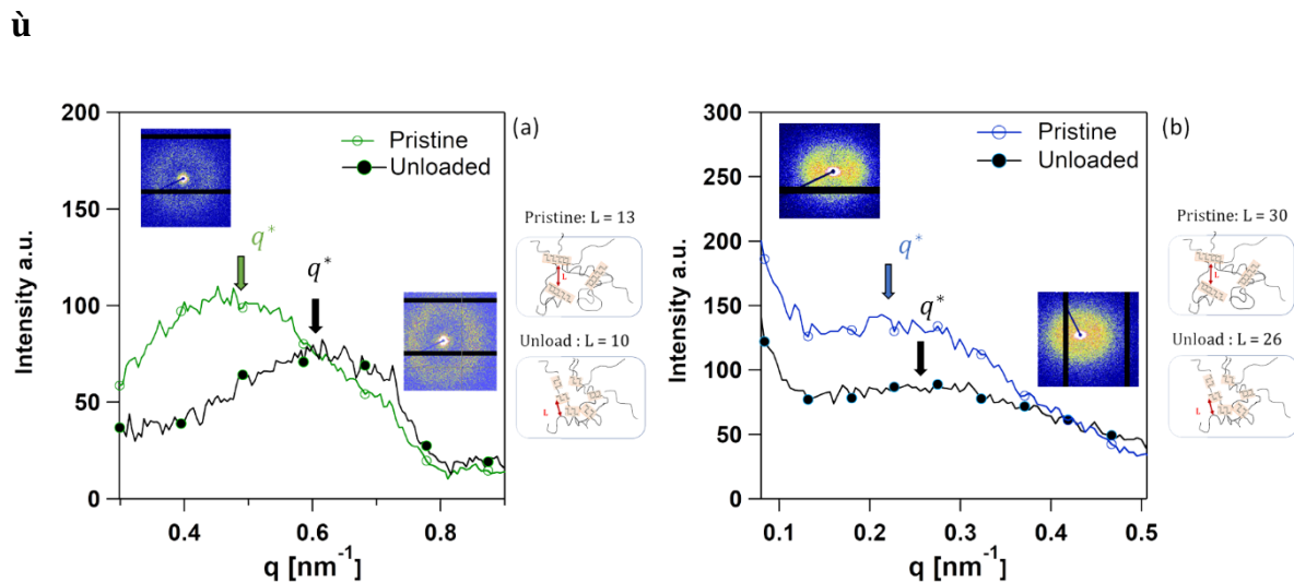
Figure 10 2D SAXS images and corresponding 1D profile for pristine and for unloaded fatigued (after 36000 cycles) TPU_XTAL (a) and TPU_SOFT(b). The schematics show the decrease of L and the fragmentation of the HD structure before and after fatigue testing (not all soft segments are represented for clarity) The X-Ray patterns were collected at DSM, The Netherlands.
