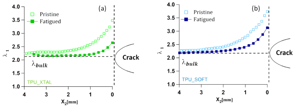
Figure 6 Maximum stretch in the loading direction \lambda_1 as a function of the distance from the open crack tip evaluated for TPU_XTAL (a) and TPU_SOFT (b), both pristine and after being fatigued for 36,000 cycles at \lambda_{max} = 2.25 .
