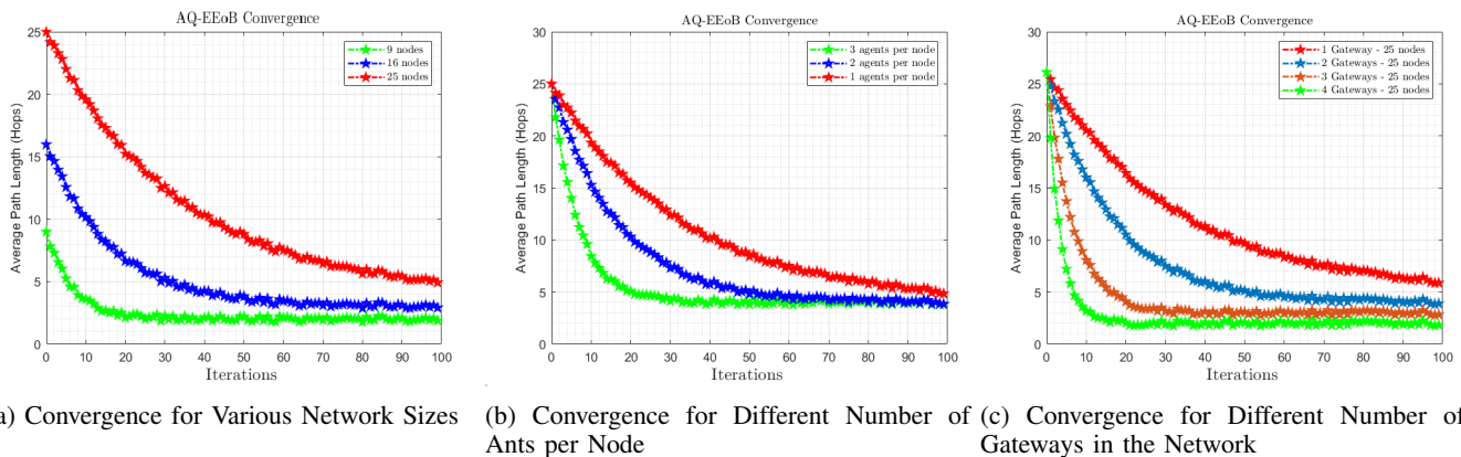
Fig. 4: AQ-EERoB convergence
