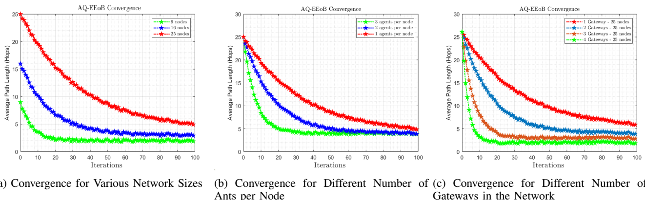
Fig. 4: AQ-EERoB convergence
