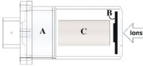
FIG. 4. Main parts of a Faraday cup
