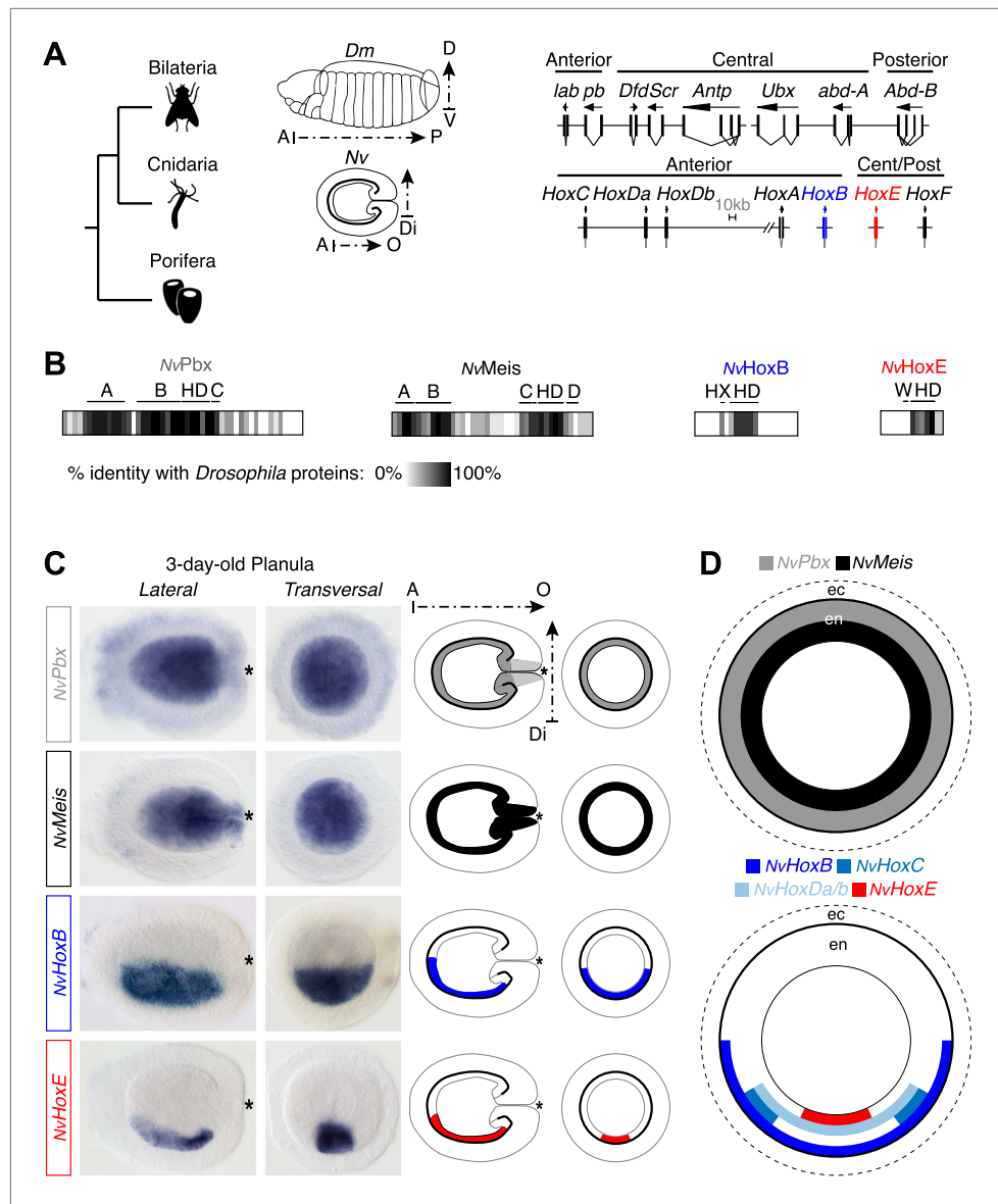
Figure 2. Hox and TALE members are co-expressed in the endoderm of the Nematostella embryo. (A) Genomic organisation of Hox genes in Nematostella vectensis (Nv) and Drosophila melanogaster (Dm), two representative species of Cnidaria and Bilateria, respectively. Embryos at the planula stage are schematized; A–P: anterior–posterior; D–V: dorsal–ventral; A–O: aboral–oral; Di: directive axis. The Nematostella embryo is oriented according to recent findings (Sinigaglia et al., 2013). The nomenclature is calqued on (Chourrout et al., 2006) to avoid confusions with bilaterian Hox paralogs: NvHoxC ( antHox7 ), NvHoxDa ( antHox8 ), NvHoxDb ( antHox8a ), NvHoxA ( antHox6 ), NvHoxB ( antHox6a ), NvHoxE ( antHox1a ), NvHoxF ( antHox1 ). The two Nematostella Hox genes under study, NvHoxB and NvHoxE, are highlighted in blue and red respectively. Note that the same colour code is used in other figures. (B) Sequence identity between Nematostella and Drosophila proteins. NvHoxB and NvHoxE are compared to Labial (Lab) and Ultrabithorax (Ubx) respectively. The percentage of identity is represented by a grayscale gradient. Conserved domains in bilaterian TALE proteins are indicated (A, B, C, D). HX: hexapeptide. HD: homeodomain. See also Figure 2—figure supplements 1–4. (C) In situ hybridization of NvPbx, NvMeis, NvHoxB and NvHoxE in a three-day-old Nematostella planula. These four genes are expressed in the endoderm (en), as illustrated in (D). Ec: ectoderm. NvPbx and NvMeis are illustrated in grey and black, respectively. This colour code is used in other figures. DOI: 10.7554/eLife.01939.004
