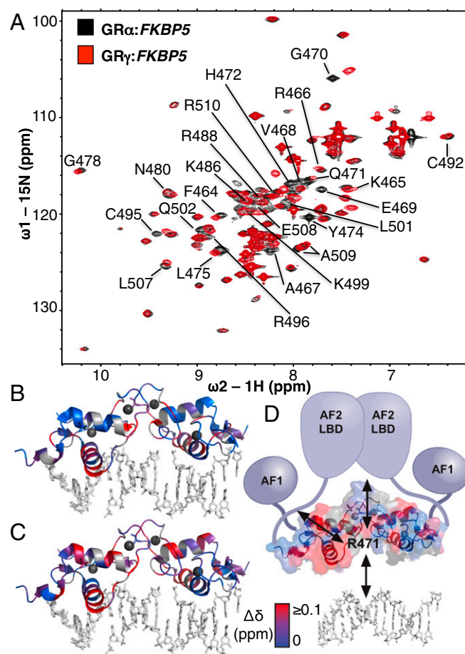
Fig. 5. Comparison of conformational changes induced by GBS or arginine insertion in the lever arm. (A) Overlay of ^1 H- ^{15} N HSQC spectra of GR \alpha (black) and GR \gamma (red) bound to FKBP5 GBS. The chemical shift difference ( \Delta\delta ) was calculated as the weighted sum of ^1 H and ^{15} N peaks for GR \alpha and GR \gamma . GR \alpha peaks with a \Delta\delta greater than the mean \Delta\delta of all peaks are labeled by residue. (B) The weighted sum of ^1 H and chemical shift differences induced by either changing GBS sequence ( ITPRIP versus FKBP5 ) or (C) arginine insertion in the lever arm (GR \alpha versus GR \gamma bound to ITPRIP ) are colored red onto the crystal structure of GR \gamma (PDB 3G6T). Blue represents residues without significant shifts. Gray represents unassigned residues. (D) Model indicating how the lever arm integrates signals from GBS variants and other functional domains of GR to influence regulatory complex composition and activity.
