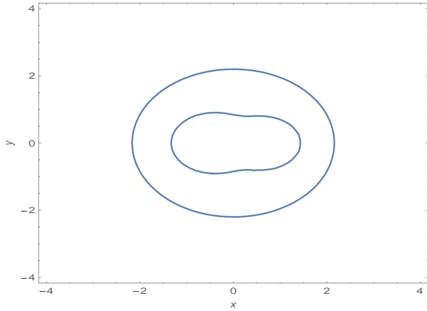
Fig. 8. Zero velocity curve when q_1 = 0.99992 , q_2 = 0.99996 , W_1 = 2.6 \times 10^{-3} , W_2 = 1.8 \times 10^{-4} , A_1 = 0.15 , A_2 = 0.2 and A_3 = 0.1
