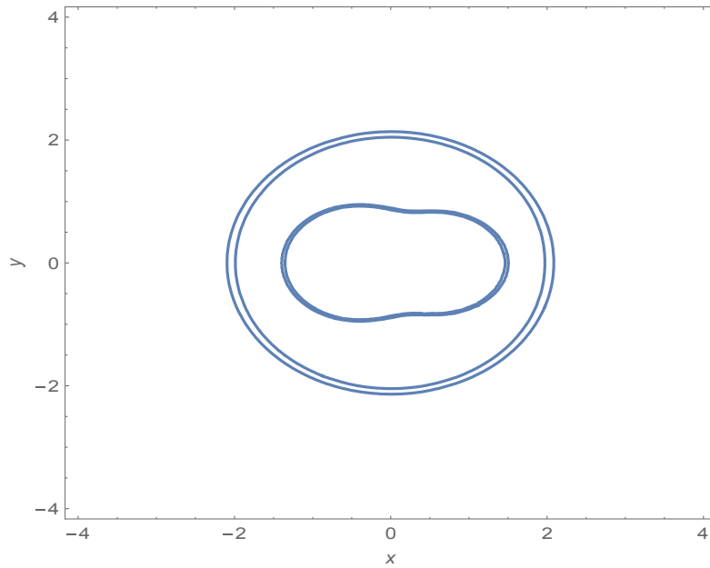
Fig. 9. Variations in the Zero velocity curves when \mu = 0.3937 , q_1 = q_2 = 1 , W_1 = W_2 = 0 , A_1 = A_2 = A_3 = 0 and when \mu = 0.3937 , q_1 = 0.99992 , q_2 = 0.99996 , W_1 = 2.6 \times 10^{-3} , W_2 = 1.8 \times 10^{-4} , A_1 = 0.15
