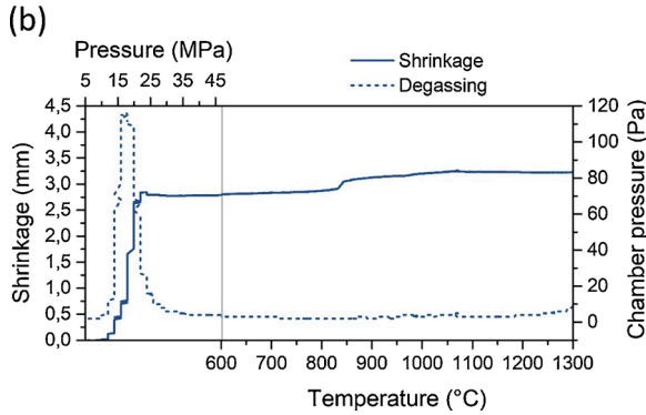
Fig. 3. High temperature dilatometry test on Spark Plasma Sintering equipment of (a) LP800 and (b) LPh.
