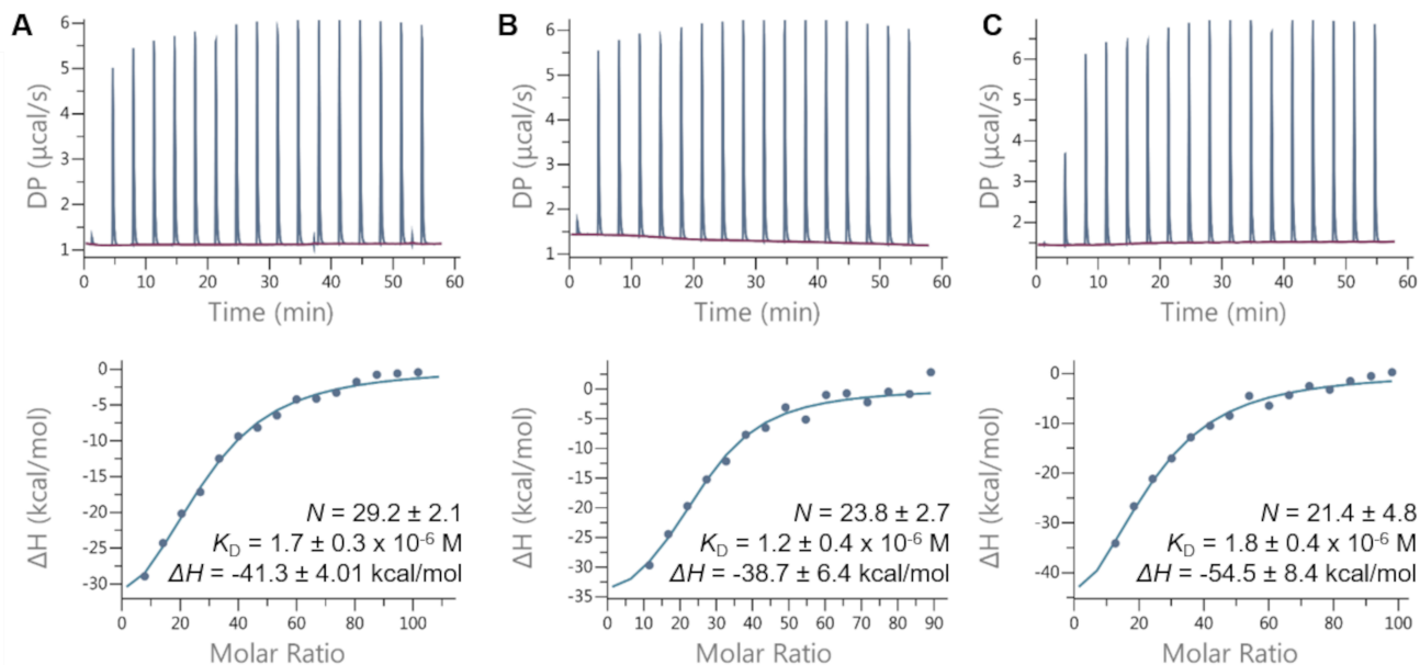
Figure 5: Isothermal titration calorimetry experiments of CCMV CPs mixed with RNA segments: B1 (A), C2 (B), and RF2 (C). Upper panels: Raw data of the heat exchange. Each spike corresponds to one injection of a CP solution ( 100 \mu\text{M} ) in a RNA solution ( 0.2 \mu\text{M} ). Lower panels: Integrated heat of each injection after subtraction of the dilution signal, and titration curve fitted according to a model of independent binding sites. Stoichiometry ( N ), dissociation constant ( K_D ), and variation of enthalpy ( \Delta H ). Each value was the average of three replicas.
