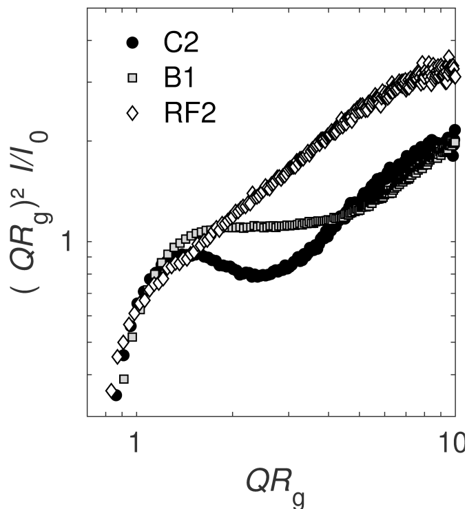
Figure 1: Small-angle X-ray scattering curves of RNA segments. RNA samples were dialyzed in a moderate ionic strength buffer (50 mM NaCl, 1 mM EDTA, 50 mM Tris-HCl pH 7.5) and their final concentration was c_{\text{RNA}} = 0.5 \text{ g.L}^{-1} . The dimensionless Kratky plot representation was chosen in order to compare the degrees of compactness. R_g is the radius of gyration, I the scattering intensity and I_0 the value of I extrapolated at Q = 0 . R_g of B1 was estimated to be 12 nm while that of C2 and RF2 was about 10 nm.
