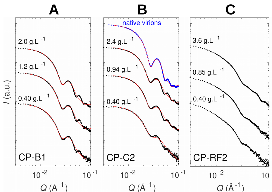
Figure 2: SAXS curves of nucleocapsids. CCMV CPs were mixed with RNAs and dialyzed in a moderate ionic strength buffer (50 mM NaCl, 50 mM Tris-HCl pH 7.5): B1 (A), C2 (B), and RF2 (C). For each system, three concentrations were measured with a CP-to-RNA mass ratio kept constant. Exact CP and RNA concentrations can be found in Table S1. Curves were fitted by a polydisperse vesicle model (solid red lines). Native virions dialyzed in the same buffer were used as a reference (blue curve).
