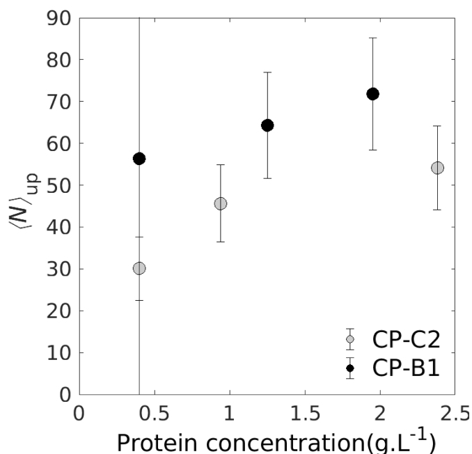
Figure 3: Mean number of bound subunits per RNA segment \langle N \rangle_{up} calculated from the scattering curves in Figure 2. CP-C2 mixtures (gray discs) and CP-B1 mixtures (black discs) of varying protein concentrations are indicated. The protein-to-RNA mass ratio was around 3.5 and 4.0 for CP-C2 and CP-B1, respectively. Error bars are standard errors of the mean.
