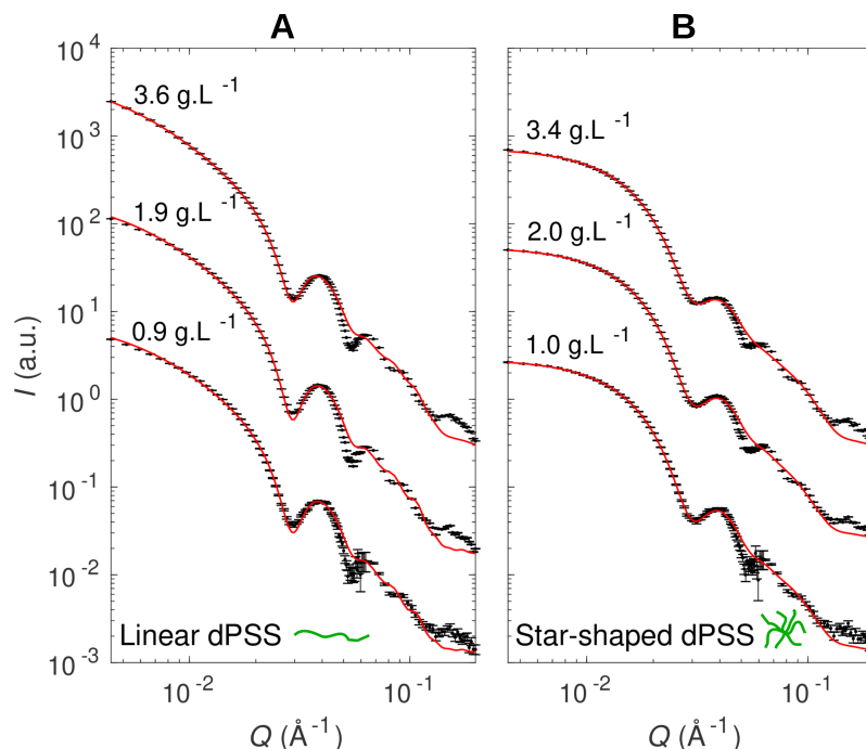
Figure 7: Effect of polyelectrolyte topology on capsid structure. SANS patterns of capsids packaging linear (A) and star (B) dPSS in 100% D 2 O in moderate ionic strength buffer (50 mM NaCl, 50 mM Tris-HCl pD 7.5). The CP concentrations are indicated next to each curve and the CP-to-PSS mass ratio was set to 6. The scattering data were fitted with a polydisperse vesicle model (red solid line; see Methods for details). The drawings illustrate the morphology of the virus-like particles with CPs in gray and dPSS in green.
