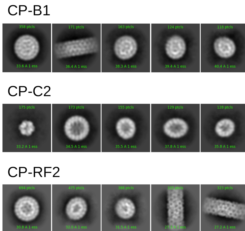
Figure 4: CryoTEM 2D classification for nucleocapsids with B1, C2 and RF2. CP concentrations were 4 \text{ g}\cdot\text{L}^{-1} , 4 \text{ g}\cdot\text{L}^{-1} and 3.6 \text{ g}\cdot\text{L}^{-1} , while CP-to-RNA mass ratios were 6, 6 and 5.5, respectively. The size of each box is 604 \text{ \AA} .
