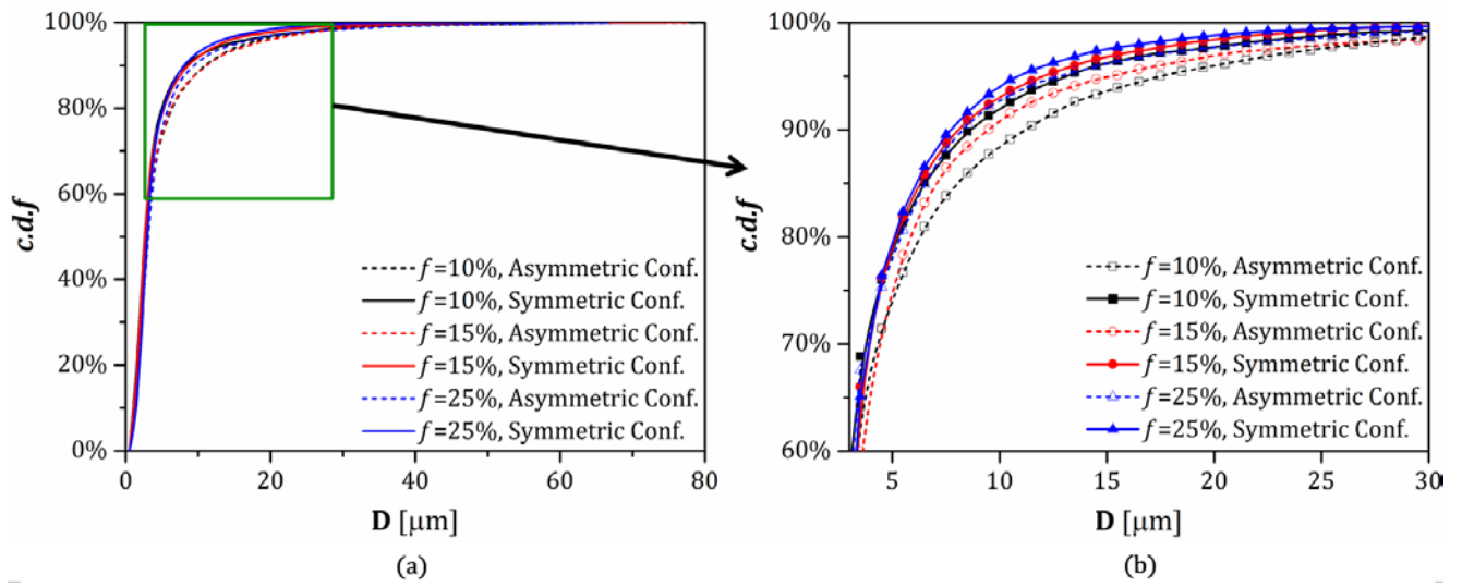
Fig.9. Cumulative distribution function of droplet diameter at Re_c=3047 : (a)[0-80 μm]; (b)[3-30 μm].
