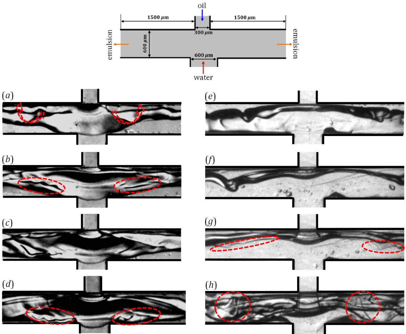
Fig.19. High-speed images of oil and water stream interactions at Re_c=1524 : (a)-(d) asymmetric configuration with f varying as 10%, 15%, 20% and 25%; (e)-(h) symmetric configuration with f varying as 10%, 15%, 20% and 25%.
