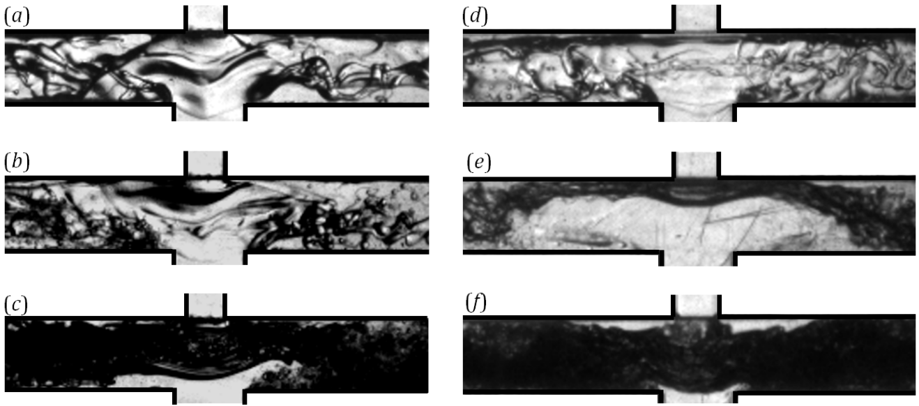
Fig.21. High speed images of oil and water stream interactions at medium and high Re conditions: (a)-(c)asymmetric configurations; (d)-(f)symmetric configurations; (a)&(d) Re_c = 3047, f = 10\% ; (b)&(e) Re_c = 4570, f = 10\% ; (c)&(f) Re_c = 4570, f = 25\% .
