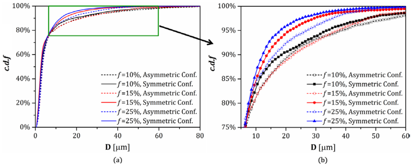
Fig.6. Cumulative distribution function of droplet diameter at Re_c = 1524 : (a) [0-80 μm]; (b) [5-60 μm].
