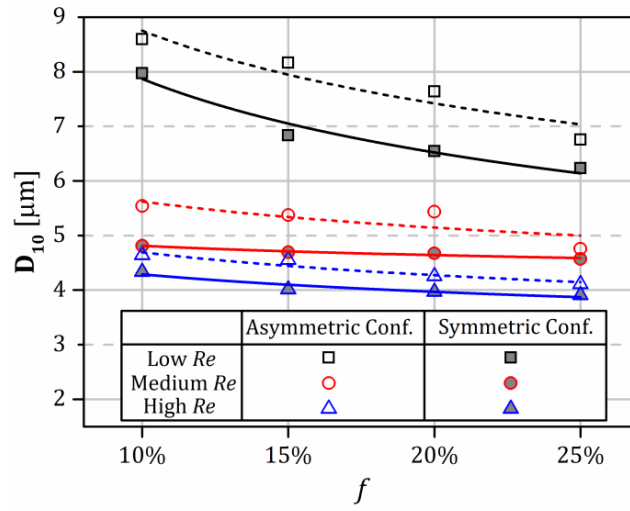
Fig.13. Arithmetic mean drop diameter for all cases.
