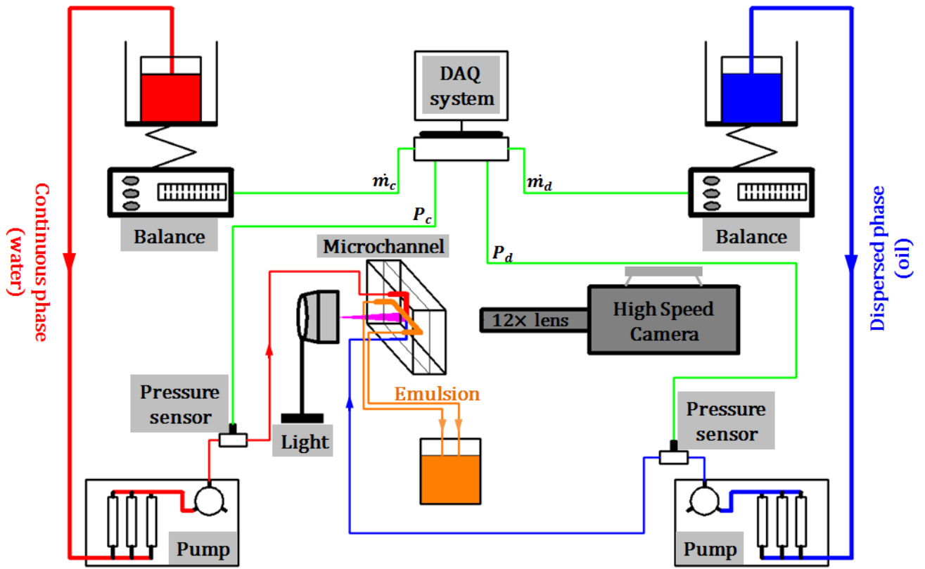
Fig. 1. Experimental setup for oil-in-water emulsification.
