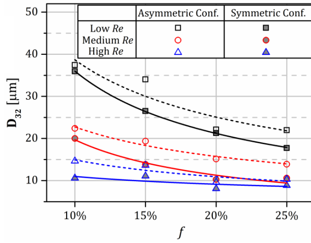
Fig.14. Sauter mean drop diameter for all cases.
