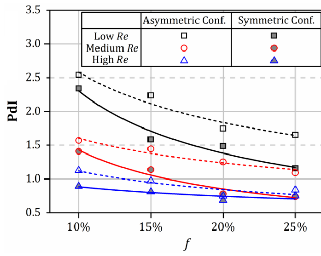
Fig.15. Polydispersity index for all cases.
