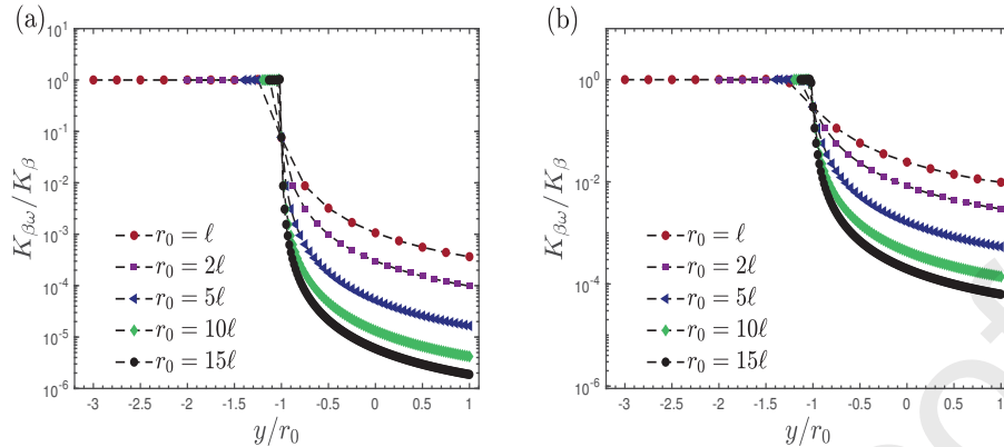
Figure 4: Spatial variations of permeabilities ratio K_{\beta\omega}/K_{\beta}(Y) in the free flow/porous medium inter-region. The porous medium model is made of a periodic array of a unit cell with a centered circle. All the calculations are obtained from the solution of the LCP taking different values of r_0 for two values of \varepsilon_{\beta\omega} : (a) 0.4 and (b) 0.8.
