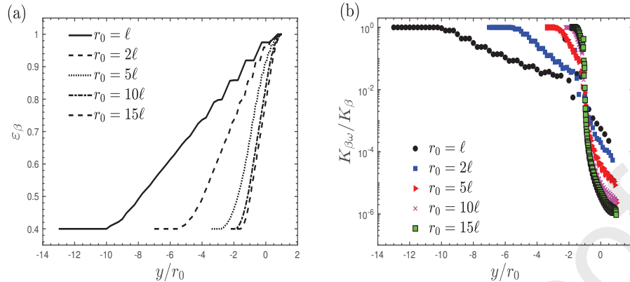
Figure 12: Spatial variations of (a) the volume fraction and (b) the permeabilities ratio K_{\beta\omega}/K_{\beta}(Y) . The porous medium consist of a periodic array of a unit cell with a centered circle which exhibit a variable particle size near the its boundaries. The prediction are obtained from filtering the pore-scale profiles taking different values of r_0 for \varepsilon_{\beta\omega} = 0.4 and \varepsilon_{max} = 0.95 . In all the calculations the whole system consist of L_{\eta} = 10^3\ell , L_{\omega} = 10^2\ell and L_S = 10\ell .
