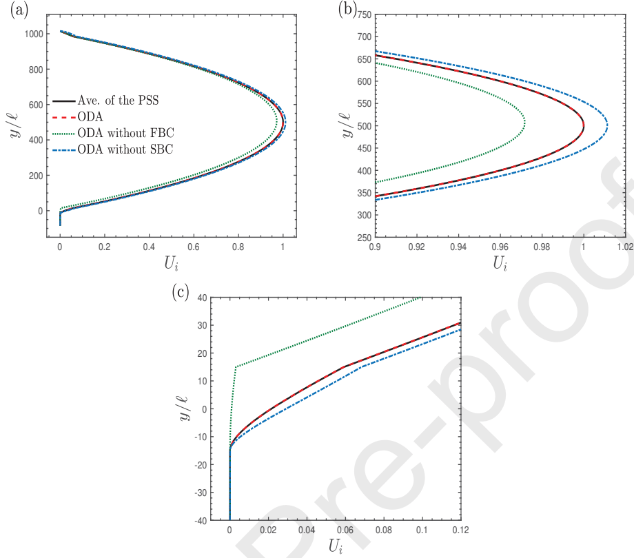
Figure 9: Comparison of intrinsic average velocity profiles in the channel partially filled with a porous medium obtained from averaging the PSS and the ODA solution (with K_\beta predicted from the PSS) by neglecting the FBC and then the SBC for r_0 = 15\ell and \varepsilon_{\beta\omega} = 0.4 . The velocity profiles are (a) in the whole channel, (b) around the maximum velocity and (c) in \eta - \omega inter-region. The porous medium model consists of a periodic array of a unit cell with a centered circle. The size of the free flow/porous medium system consists of L_\eta = 10^3\ell and L_\omega = 10^2\ell .
