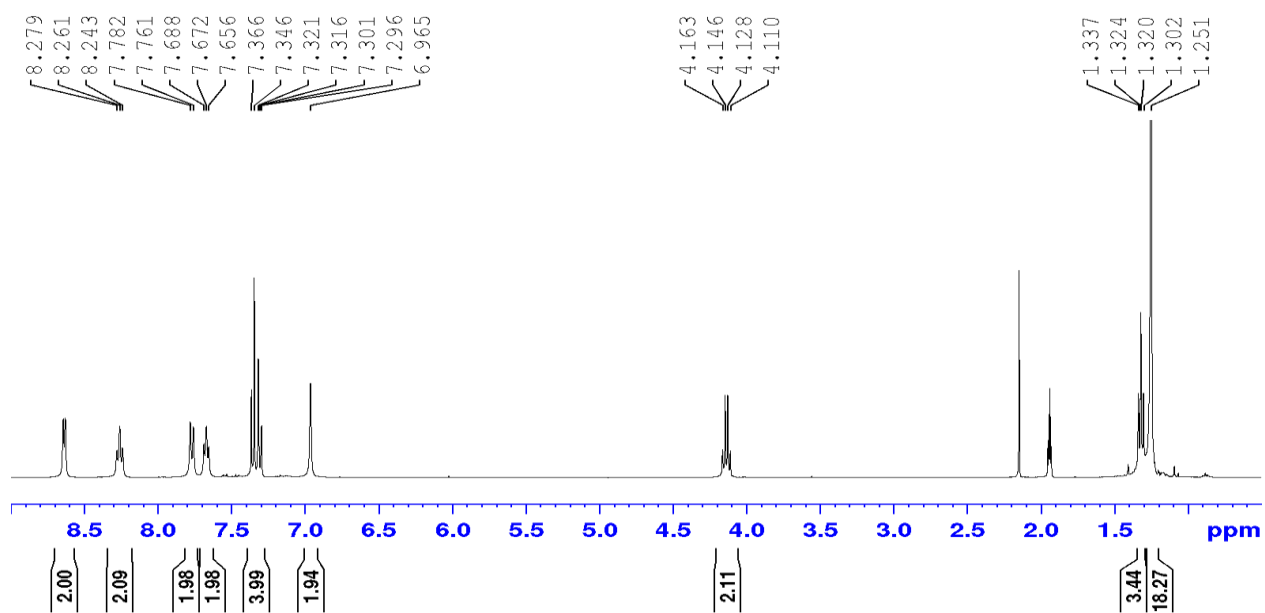
Figure S25: ^1\text{H} NMR spectrum of 8 in \text{CD}_3\text{CN} at 298 K.
