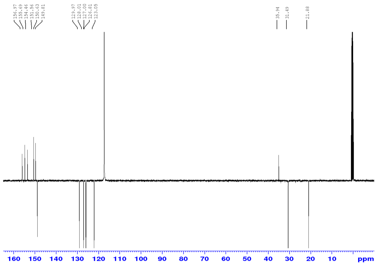
Figure S12: Jmod ^{13}\text{C}\{^1\text{H}\} NMR spectrum of 2a in \text{CD}_3\text{CN} at 298 K.
