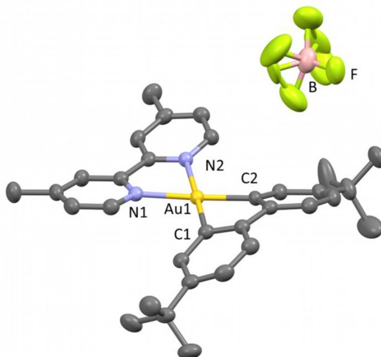
Figure S2: Crystal structure of complex 2a . Ellipsoids set at 50% probability. Hydrogen atoms and toluene have been omitted for clarity. Selected bond distances [Å] and angles [°] measured at 140K: Au 1 -C 1 2.021(3), Au 1 -C 2 2.029(3), Au 1 -N 1 2.130(2), Au 1 -N 2 2.132(2), N 1 -Au 1 -N 2 76.83(9), N 2 -Au 1 -C 2 102.1(1), C 2 -Au 1 -C 1 79.2(1) C 1 -Au 1 -N 1 101.7(1).
