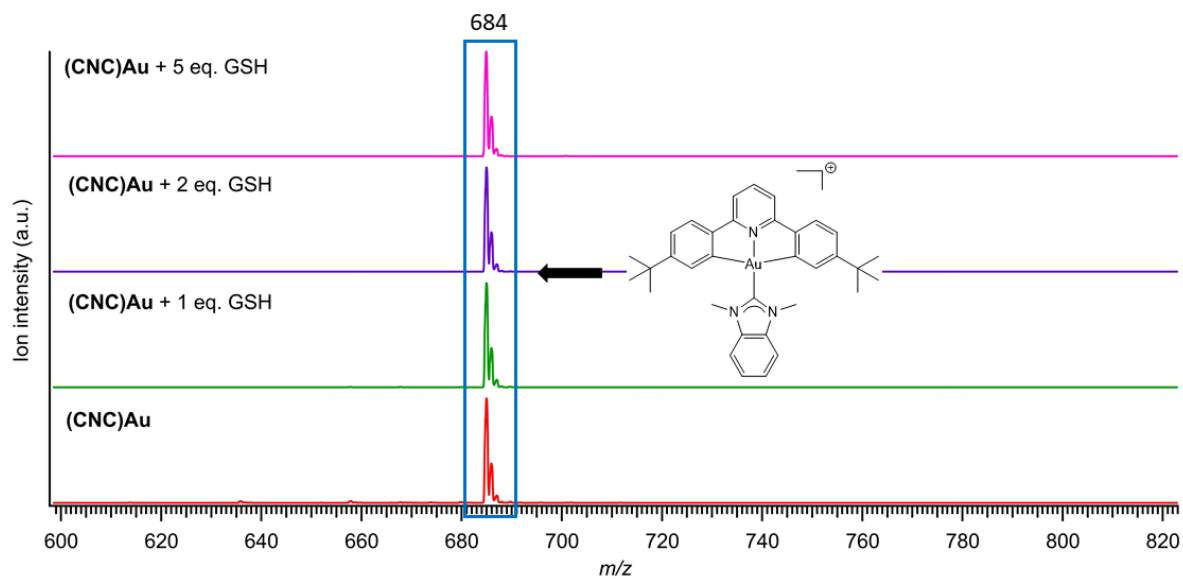
Figure S7: ESI(+)-MS of complex (CNC)Au alone or in solution with 1, 2 or 5 equivalents of GSH recorded after 24 h of incubation at 37 °C in DMSO/PBS 1:1.
