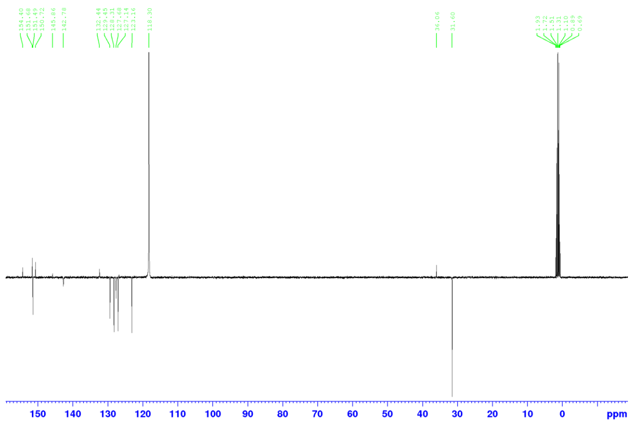
Figure S17: Jmod ^{13}\text{C}\{^1\text{H}\} NMR spectrum of 4 in \text{CD}_3\text{CN} at 298 K.
