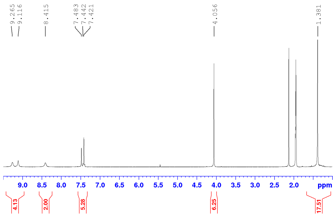
Figure S14: ^1\text{H} NMR spectrum of 3 in \text{CD}_3\text{CN} at 298 K.
