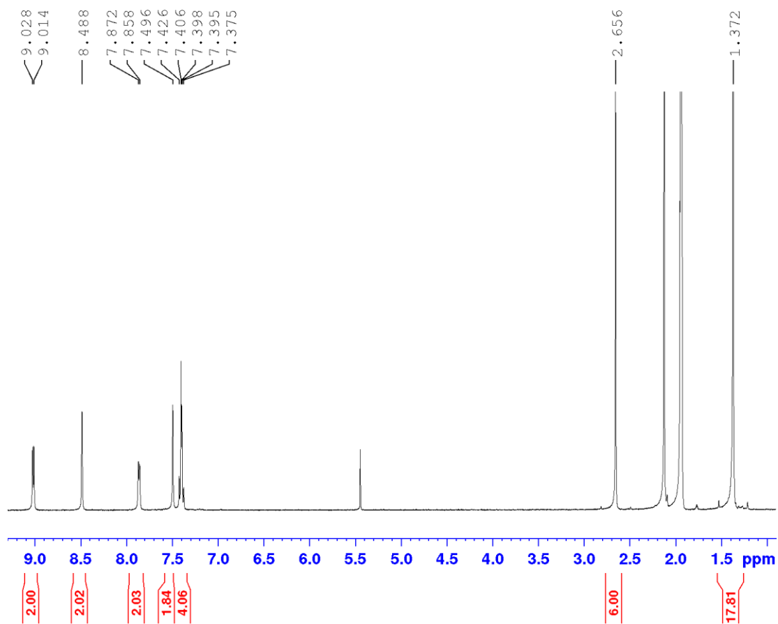
Figure S11: ^1\text{H} NMR spectrum of 2a in \text{CD}_3\text{CN} at 298 K.
