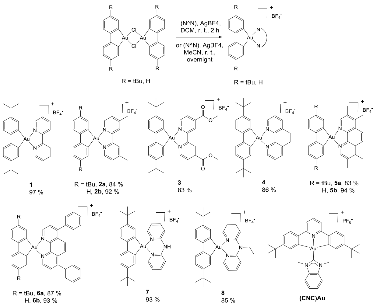
Figure 3: Synthesis and structure of [(C^C)Au(N^N)]BF_4 complexes 1-8 and ( CNC )Au.
