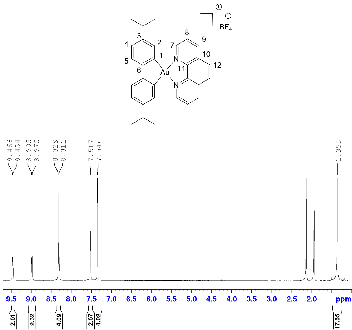
Figure S16: ^1\text{H} NMR spectrum of 4 in \text{CD}_3\text{CN} at 298 K.
