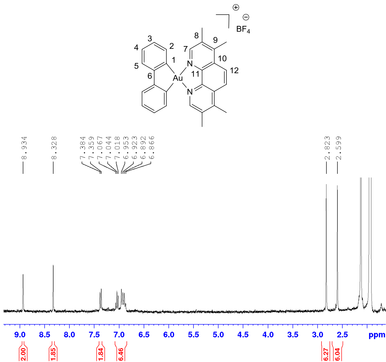
Figure S20: ^1\text{H} NMR spectrum of 5b in \text{CD}_3\text{CN} at 298 K.
