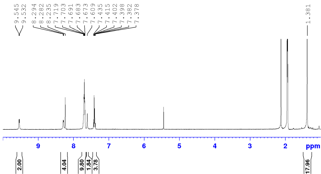
Figure S21: ^1\text{H} NMR spectrum of 6a in \text{CD}_3\text{CN} at 298 K.
