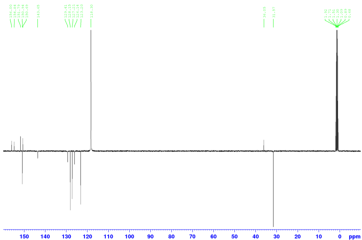
Figure S10: Jmod ^{13}\text{C}\{^1\text{H}\} NMR spectrum of 1 in \text{CD}_3\text{CN} at 298 K.
