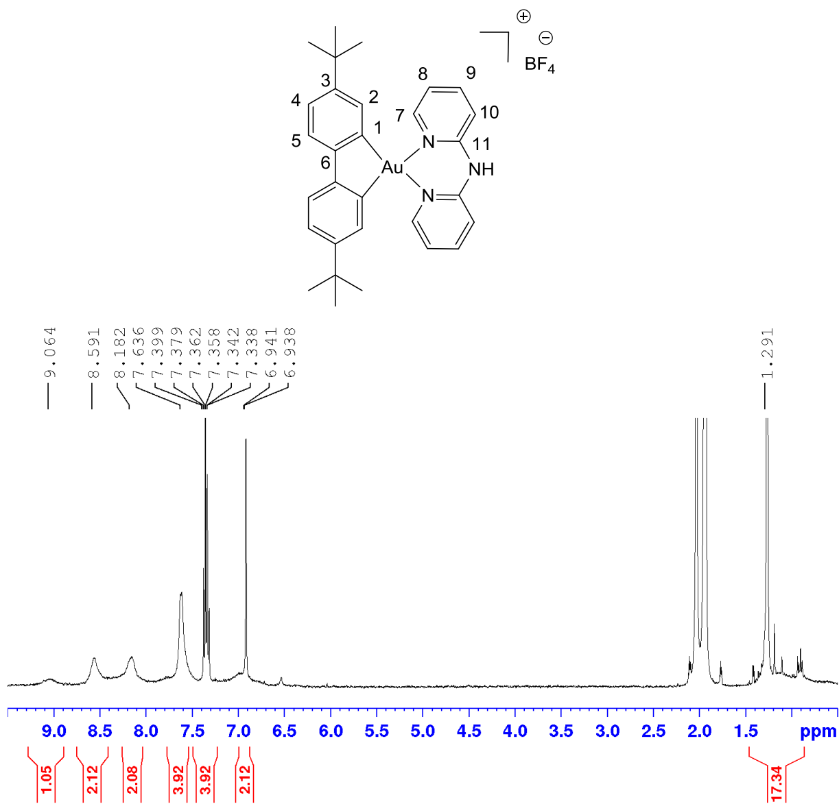
Figure S24: ^1\text{H} NMR spectrum of 7 in \text{CD}_3\text{CN} at 323 K.
