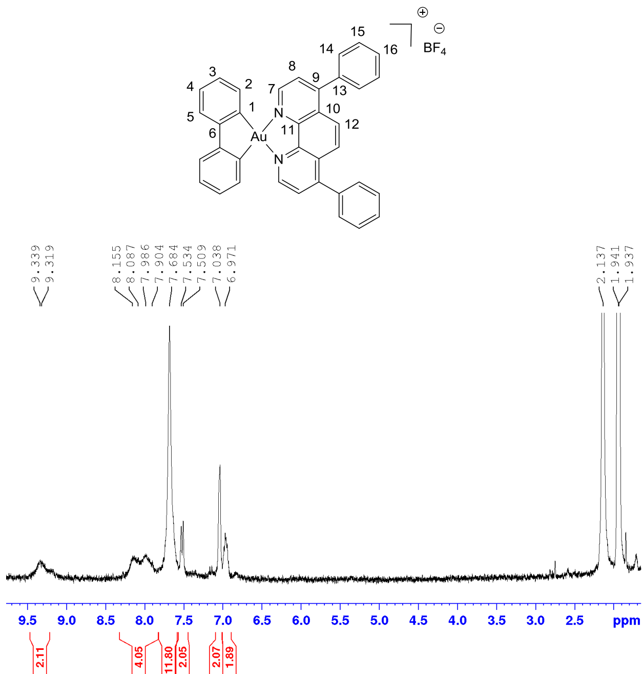
Figure S23: ^1\text{H} NMR spectrum of 6b in \text{CD}_3\text{CN} at 323 K.
