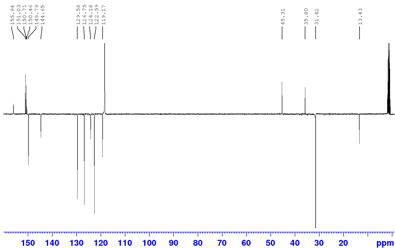
Figure S26: Jmod ^{13}\text{C}\{^1\text{H}\} NMR spectrum of 8 in \text{CD}_3\text{CN} at 298 K.
