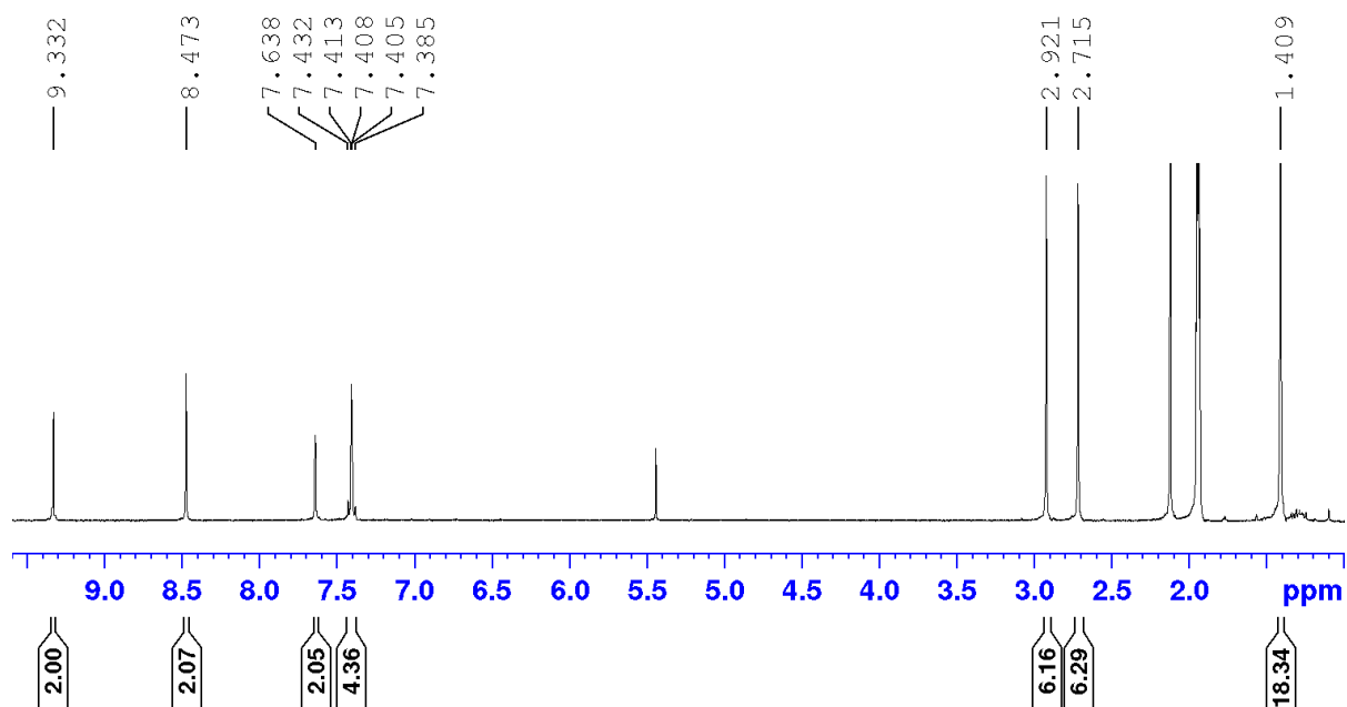
Figure S18: ^1\text{H} NMR spectrum of 5a in \text{CD}_3\text{CN} at 298 K.
