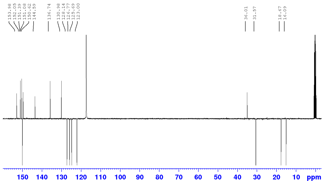
Figure S19: Jmod ^{13}\text{C}\{^1\text{H}\} NMR spectrum of 5a in \text{CD}_3\text{CN} at 298 K.
