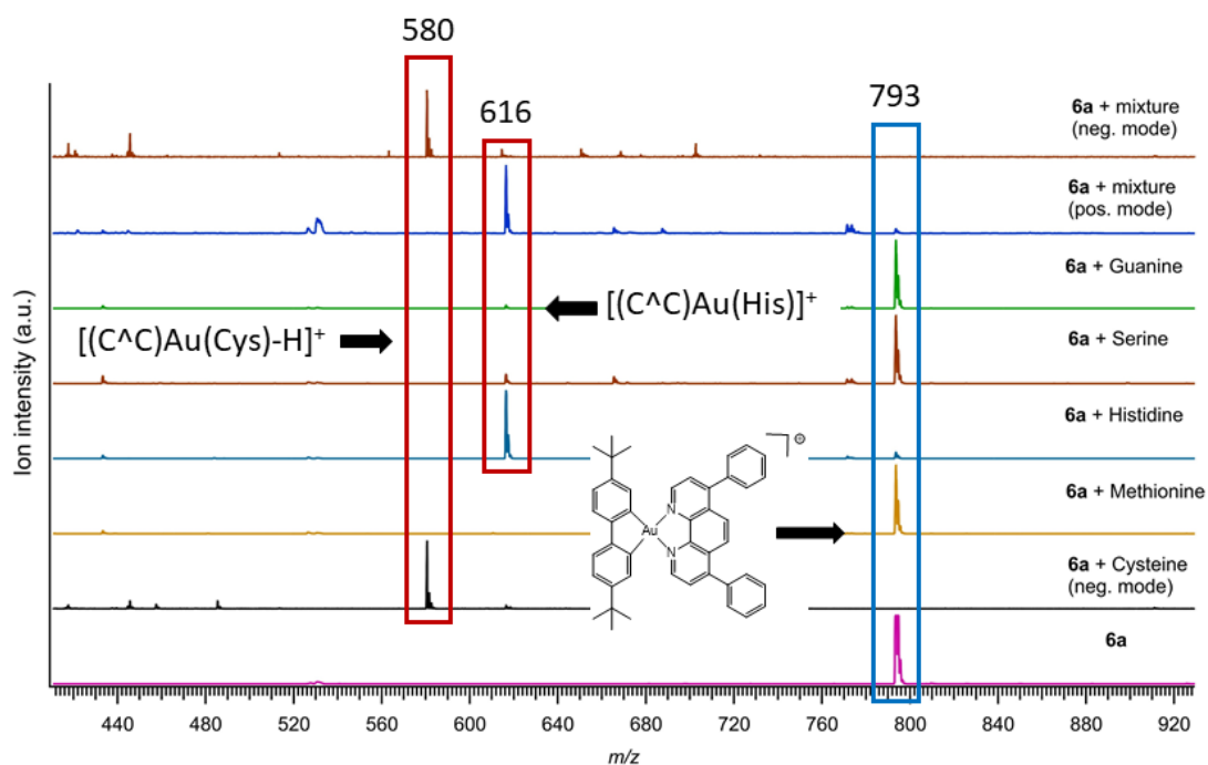
Figure S4: ESI-MS in negative or positive modes of complex 6a alone or in solution with 1 eq. amino acids and/or guanine recorded after 24 h of incubation at 37 °C in DMSO.
