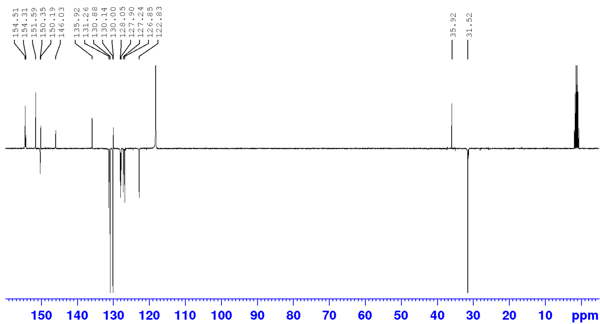
Figure S22: Jmod ^{13}\text{C}\{^1\text{H}\} NMR spectrum of 6a in \text{CD}_3\text{CN} at 298 K.
