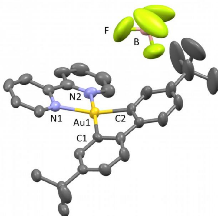
Figure S1: Crystal structure of complex 1 . Ellipsoids set at 50% probability. Hydrogen atoms have been omitted for clarity. Selected bond distances [ \text{\AA} ] and angles [ ^\circ ] measured at 140K: \text{Au}_1\text{-C}_1 2.03(1), \text{Au}_1\text{-C}_2 2.028(9), \text{Au}_1\text{-N}_1 2.131(7), \text{Au}_1\text{-N}_2 2.144(7), \text{N}_1\text{-Au}_1\text{-N}_2 76.9(3), \text{N}_2\text{-Au}_1\text{-C}_2 103.5(3), \text{C}_2\text{-Au}_1\text{-C}_1 80.3(3) \text{C}_1\text{-Au}_1\text{-N}_1 103.5(3).
