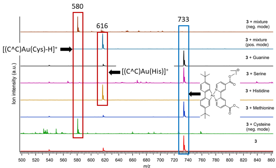
Figure S3: ESI-MS in negative or positive modes of complex 3 alone or in solution with 1 eq. amino acids and/or guanine recorded after 24 h of incubation at 37 °C in DMSO.
