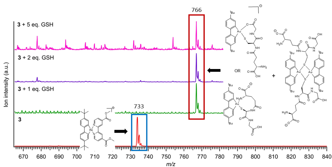
Figure S5: ESI(-)-MS of complex 3 alone or in solution with 1, 2 or 5 equivalents of GSH recorded after 24 h of incubation at 37 °C in DMSO/PBS 1:1.
