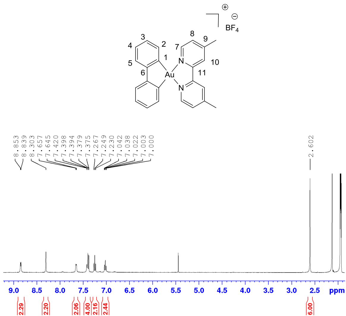
Figure S13: ^1\text{H} NMR spectrum of 2b in \text{CD}_3\text{CN} at 298 K.
