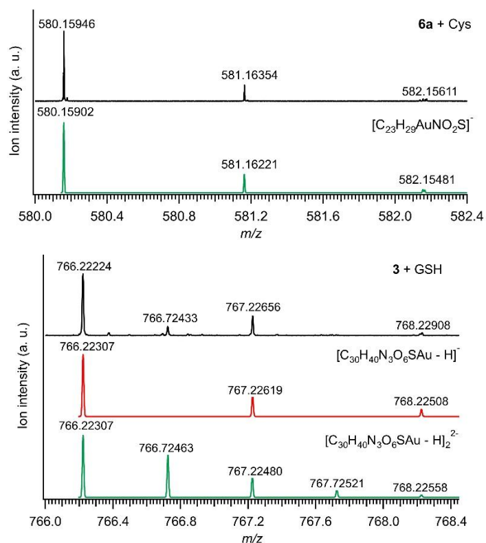
Figure S6: HRMS and corresponding isotopic patterns of the association complexes of 3 and 6a with histidine, cysteine and GSH (in positive or negative mode) observed after 24 h of incubation at 37 °C in DMSO/PBS 1:1.
