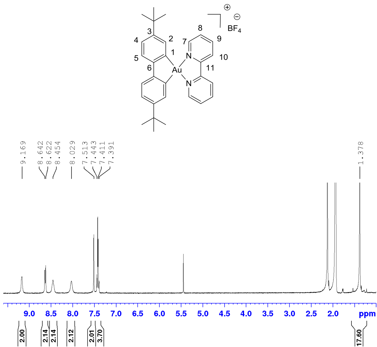
Figure S9: ^1\text{H} NMR spectrum of 1 in \text{CD}_3\text{CN} at 298 K.
