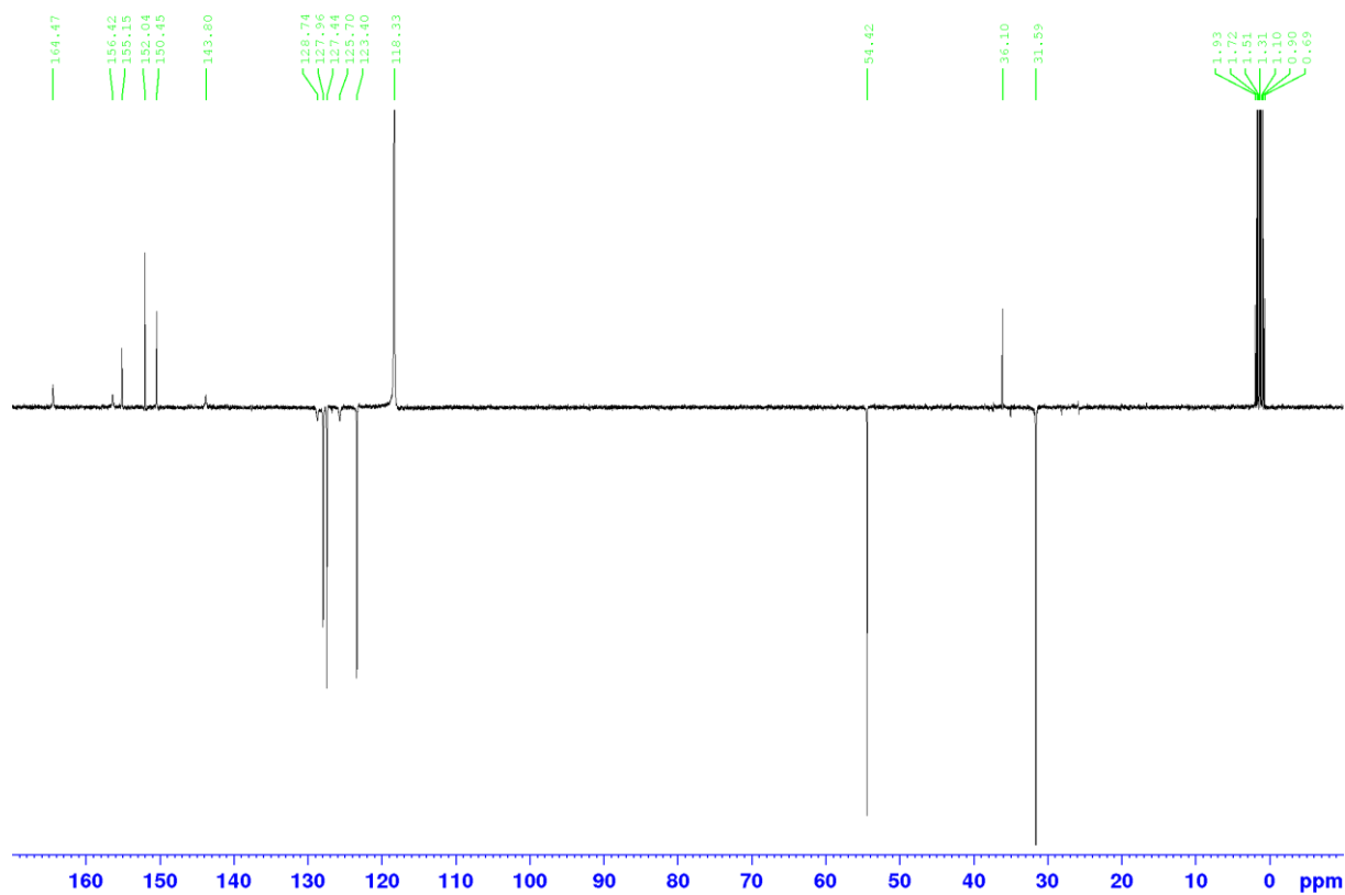
Figure S15: Jmod ^{13}\text{C}\{^1\text{H}\} NMR spectrum of 3 in \text{CD}_3\text{CN} at 298 K.
