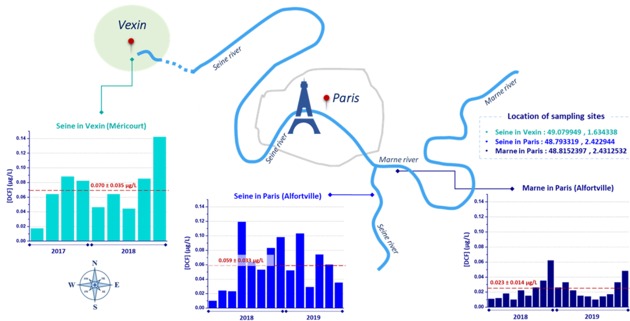
Figure 6. Sampling sites of surface water collected in the Marne river in Paris and the Seine river in Paris and Vexin; and corresponding DCF concentrations determined by eaufrance agency 38 with average values.
