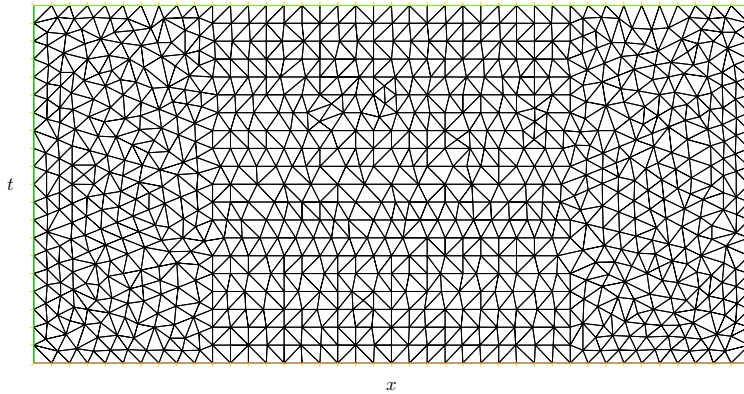
Figure 1: Regular space-time mesh of Q_T := (0, 1) \times (0, T) composed of 1744 triangles and 933 vertices; h \approx 0.0208 .
