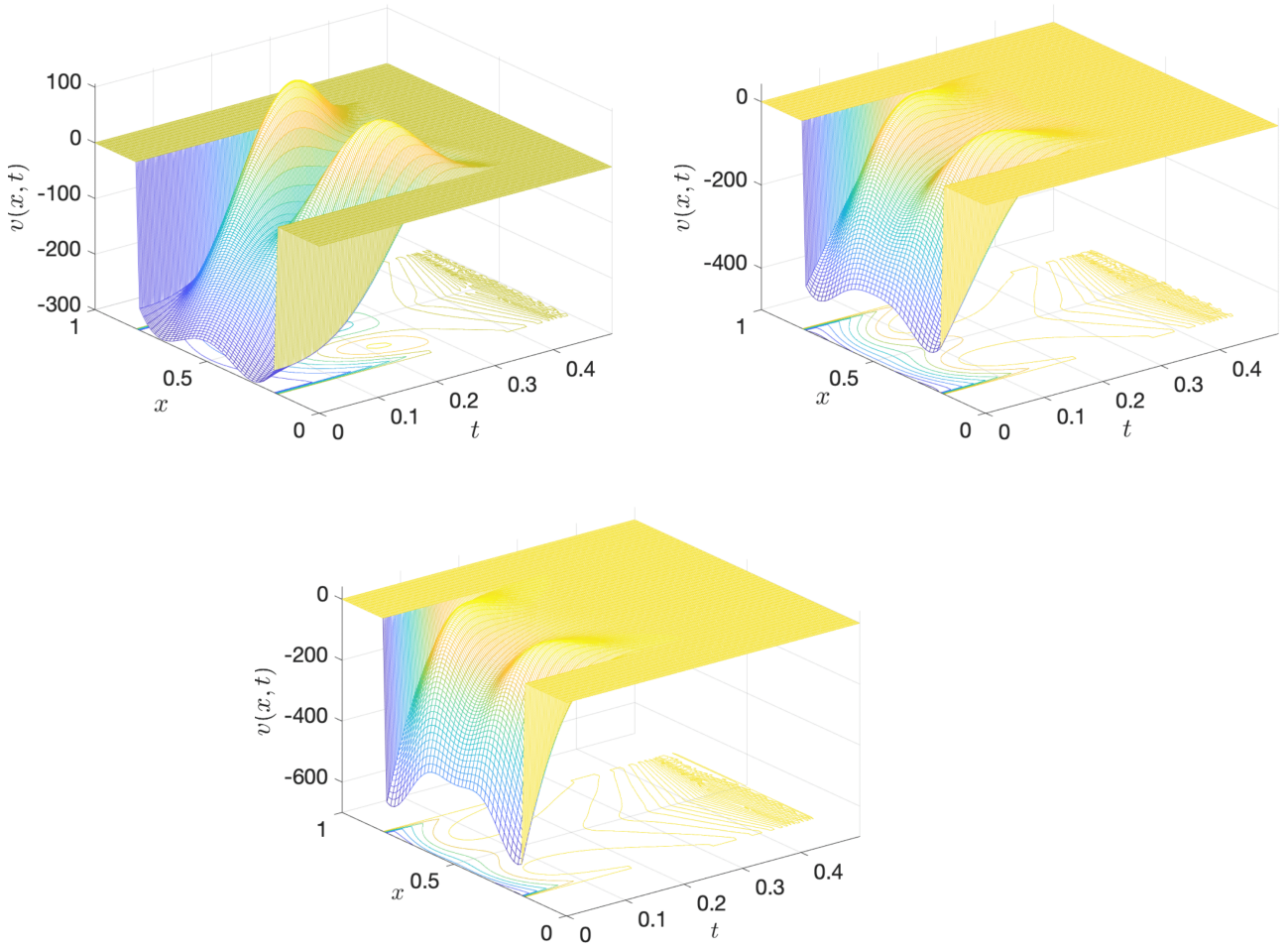
Figure 4: The control v_{k^*} in Q_T for c_{u_0} = 10 , c_f = -5 and s \in \{1, 2, 3\} .
