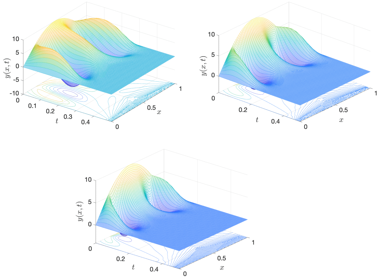
Figure 5: The controlled solution y_{k^*} in Q_T for c_{u_0} = 10 , c_f = -5 and s \in \{1, 2, 3\} .
