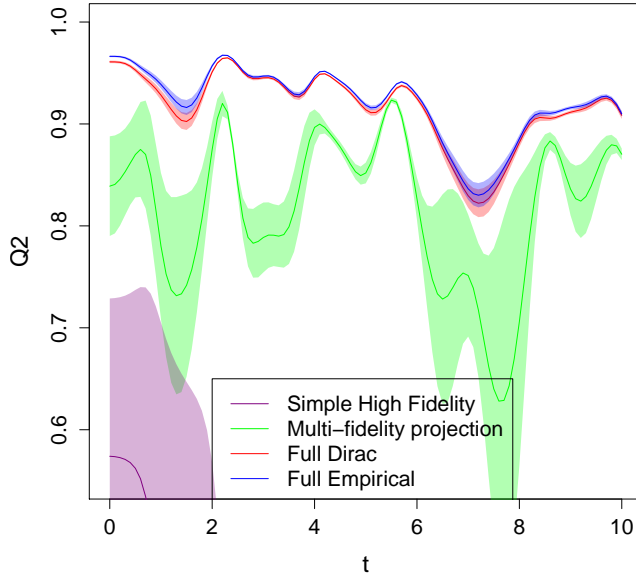
FIGURE 6.3. Comparison between the methods in terms of time-dependent Q^2 . Averages over 40 random experimental designs are computed. The colored fields represent the confidence intervals determined by \pm 1.96 standard deviation. Here N_H = 10 , N_L = 100 and N_t = 101 .
