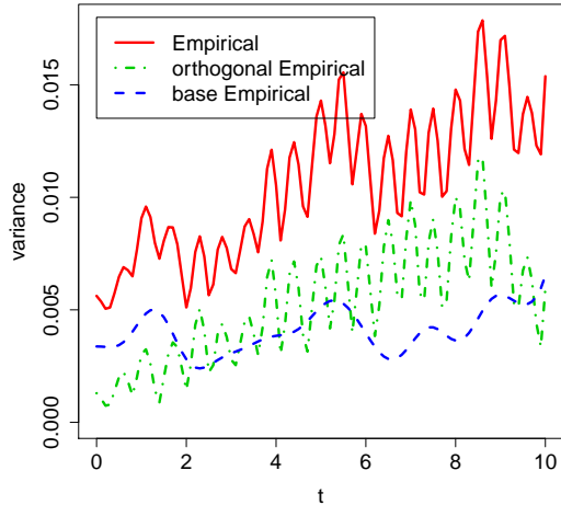
FIGURE 6.5. Estimation of the different time-dependent prediction variance terms for the empirical basis method.
