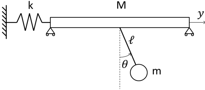
FIGURE 6.1. The double pendulum system with its parameters.
