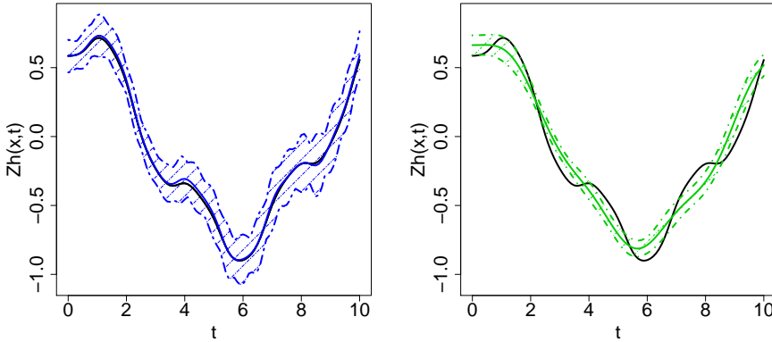
FIGURE 6.4. Comparison between the predictions of the full method (left) and the dimension reduction only method (right). The black solid line is the exact high-fidelity time series, the colored solid line is the prediction mean and the dashed lines are the confidence intervals. In this example the value of N obtained by cross validation is 8.
