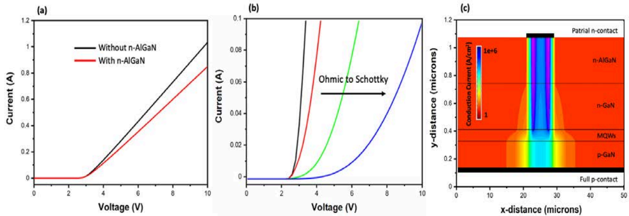
Figure 4. (a) Simulated current-voltage characteristics of VTF-LEDs with and without the n-AlGaIn layer. (b) Simulated effect of the Schottky n-contact on the current-voltage characteristic of VTF-LEDs. (c) Current distribution in a VTF-LED without mesa isolation.
