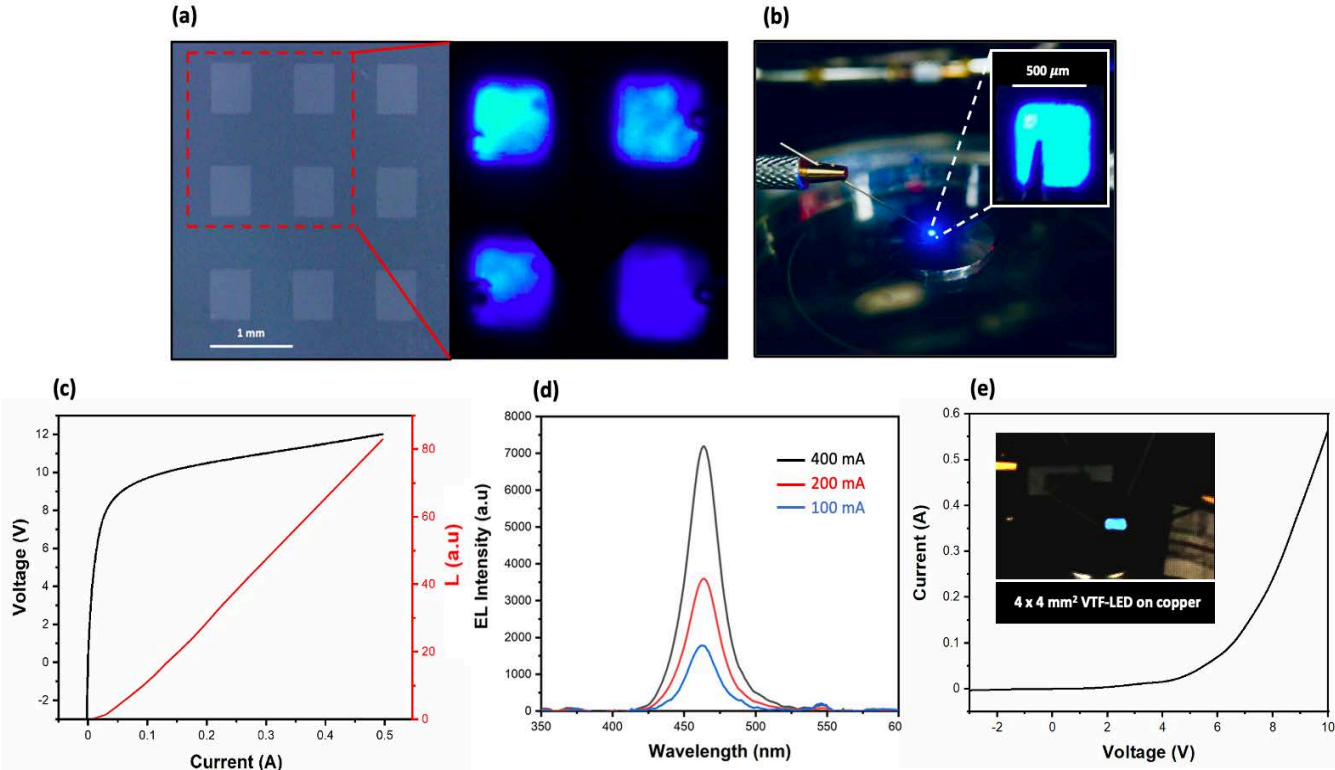
Figure 3. (a) Electroluminescence image of 4 VTF-LEDs connected in parallel and operated at 8V. (b) Photographs of a homogeneous VTF-LED operated at 300 mA. (c) Current-voltage and optical power versus current characteristics of the VTF-LED in (b). (d) Electro-luminescence spectra of the VTF-LED for different levels of injected current. (e) Current-voltage of a large size (4 mm x 4 mm) VTF-LED. Inset is a photograph of this LED operated at 500 mA.
