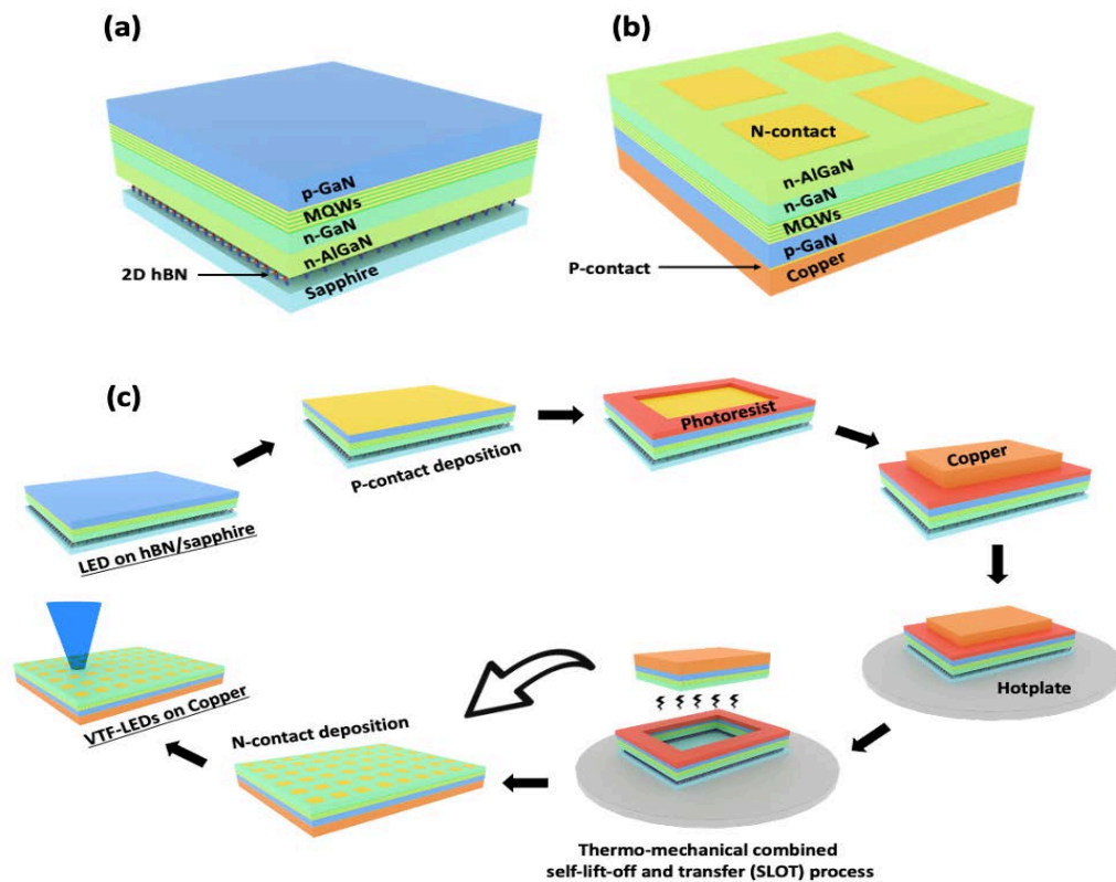
Figure 1. Schematics of (a) LEDs structure grown on hBN/sapphire, (b) VTF-LEDs on copper fabricated by SLOT process and (c) different steps of the SLOT process for fabrication of VTF-LEDs.
