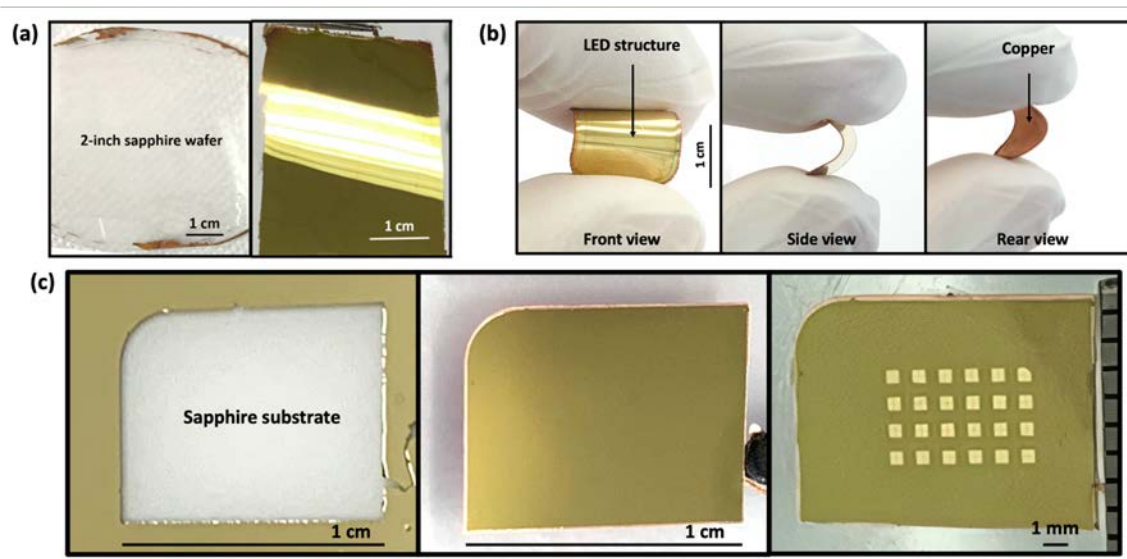
Figure 2. (a) Photographs of 4 x 3 cm 2 LED membrane and the corresponding sapphire substrate after the membrane release using the SLOT process (the bright stripe on the membrane corresponds to the reflection of the ceiling neon lamp in the cleanroom). (b) Photographs of a 1-cm 2 membrane, highlighting its bending possibility. (c) Photographs of a 1-cm 2 released membrane on which an array of 0.5 x 0.5 mm 2 VTF-LEDs is fabricated.
