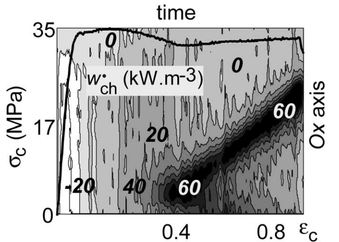
Fig. 1. Time evolution of the longitudinal heat source profile w_{ch}^{\bullet}(x, 0, t) . The test is velocity-controlled ( = 0.05 \text{ mm}\cdot\text{s}^{-1} ).
